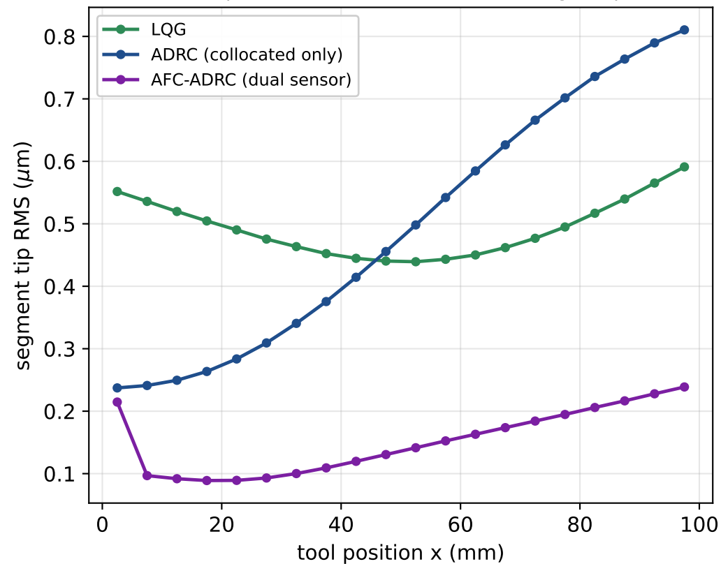
(a) final pass ( h = 3.0 mm): vibration along the path
