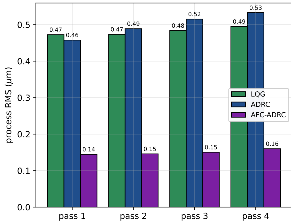
(b) per-pass process RMS
