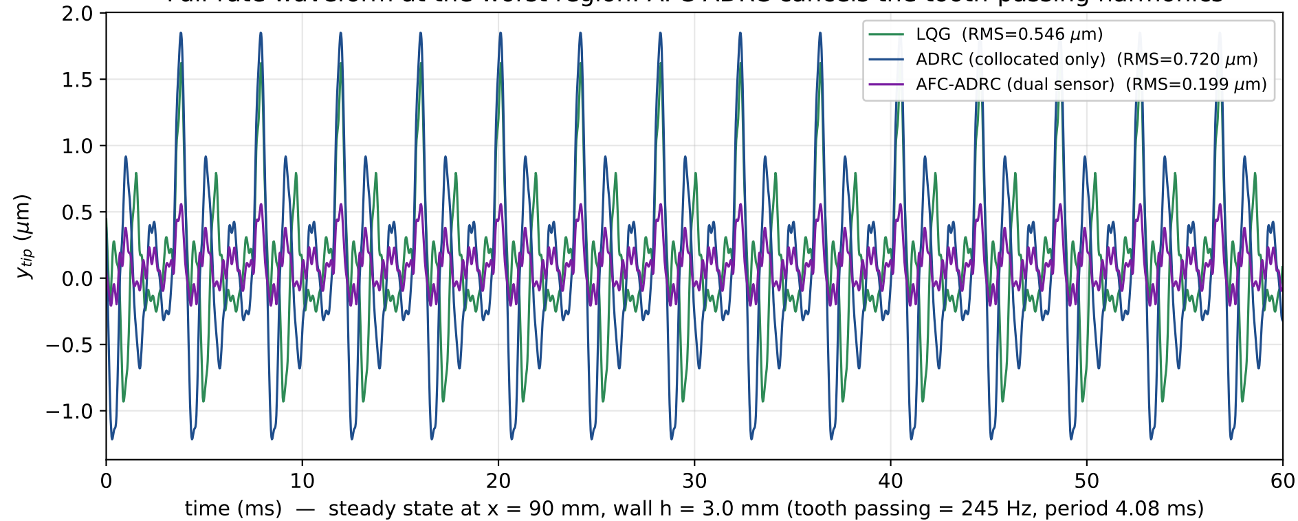
Full-rate waveform at the worst region: AFC-ADRC cancels the tooth-passing harmonics
