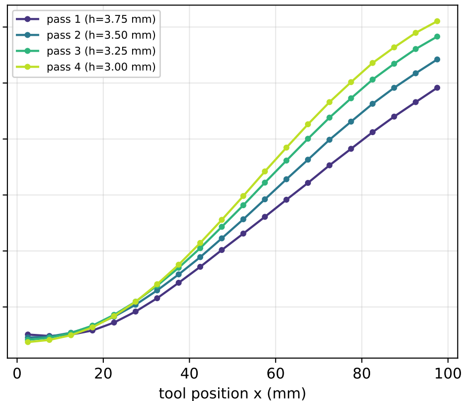
ADRC (frozen design) per-pass RMS: 0.46, 0.49, 0.52, 0.53 \mu\text{m}
