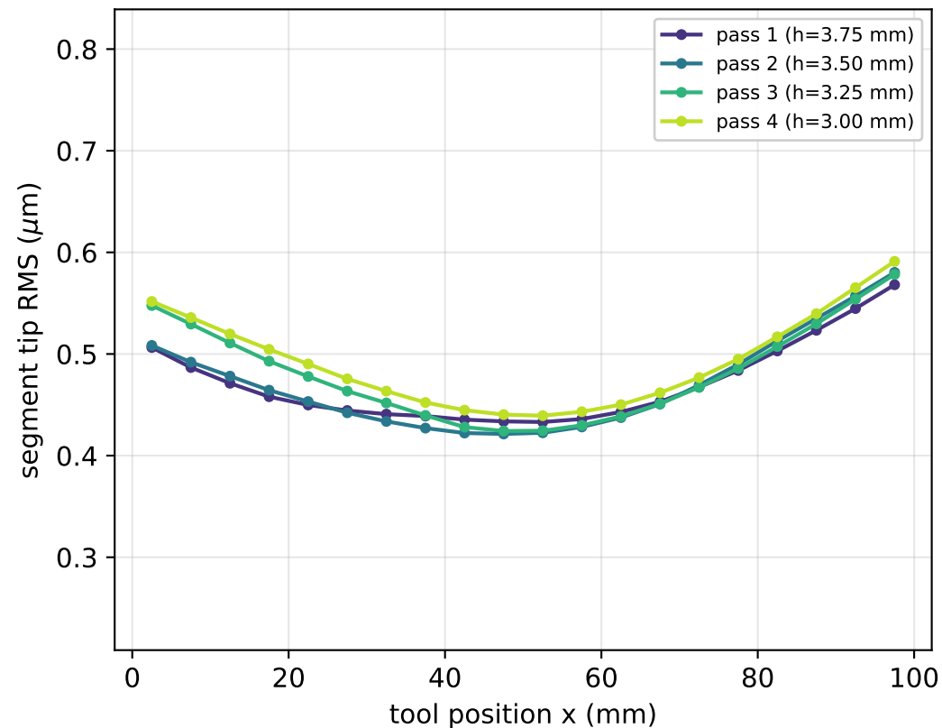
LQG (frozen design) per-pass RMS: 0.47, 0.47, 0.48, 0.49 \mu\text{m}
