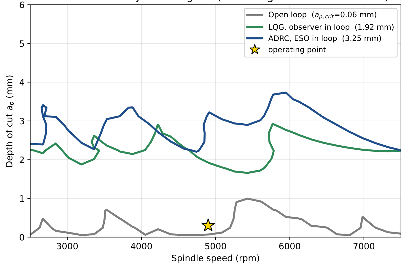
Controlled stability-lobe diagram (stable region below each curve)
