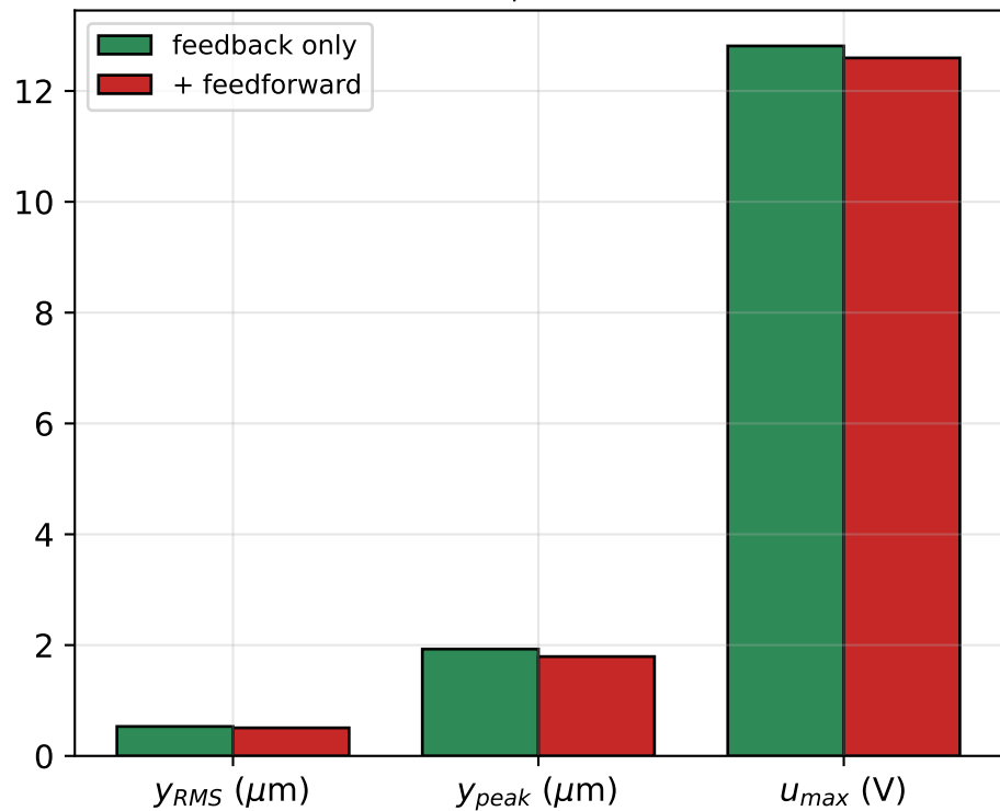
(b) role of feedforward ( a_{p,crit} unchanged = 2.43 mm)
