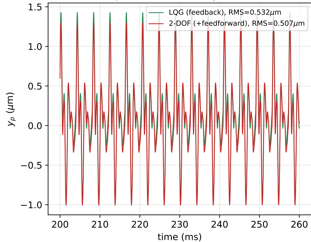
(a) S1 tip vibration (steady-state zoom)
