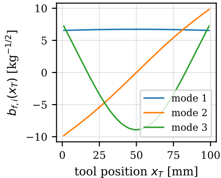
(a) modal participation along path
