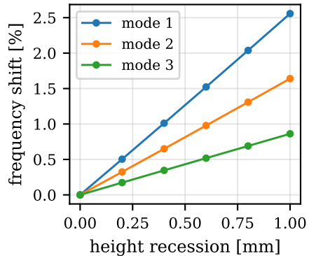
(c) material-removal drift
