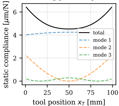
(b) milling-point compliance
