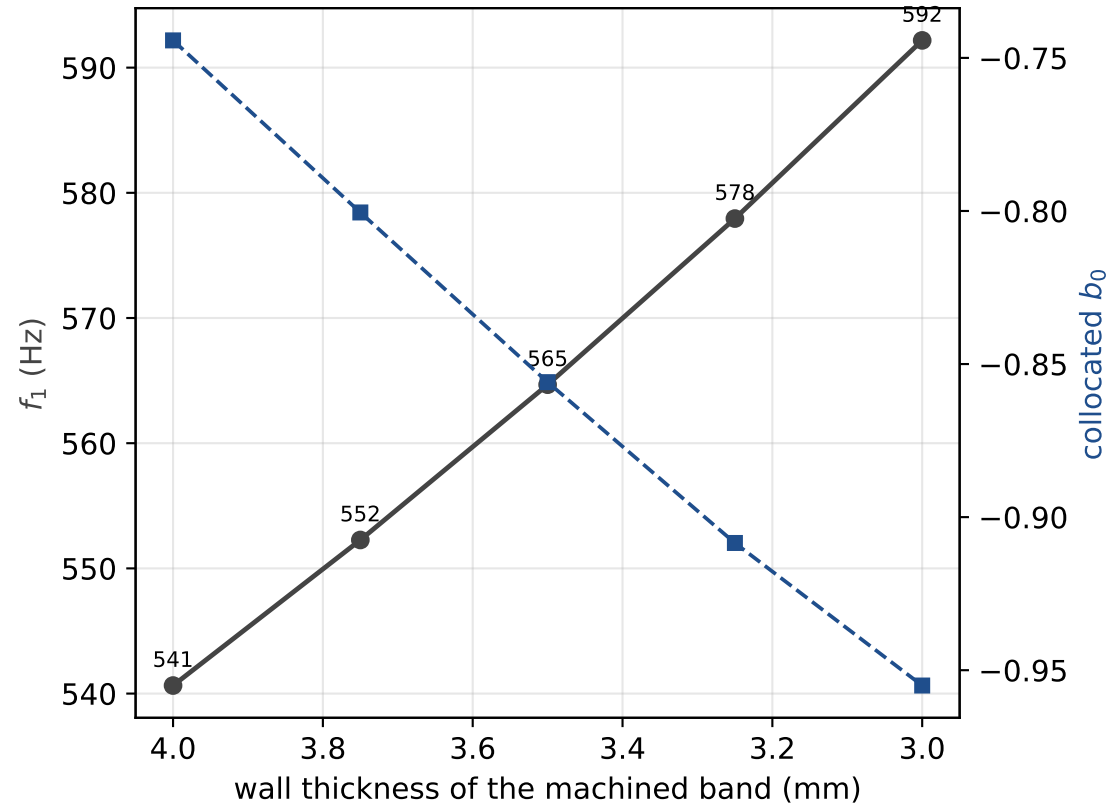
(a) modal drift from material removal (single pass < 0.017 %; thinning +9.5 %)
