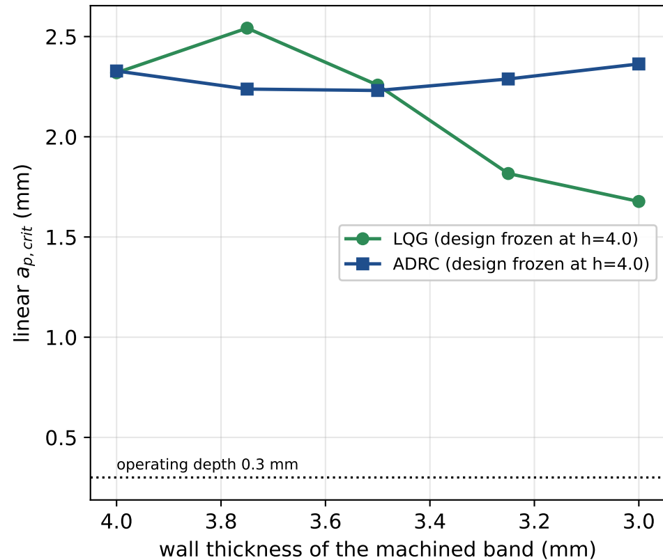
(b) frozen designs across the machining process (x / + = chatter at the 0.3 mm operating point)
