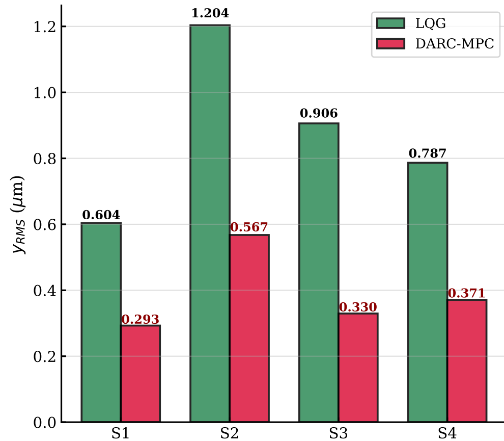
(a) RMS vibration
