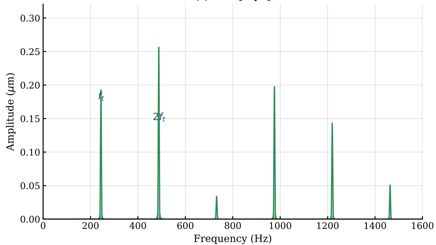
(c) FFT[LQG]
