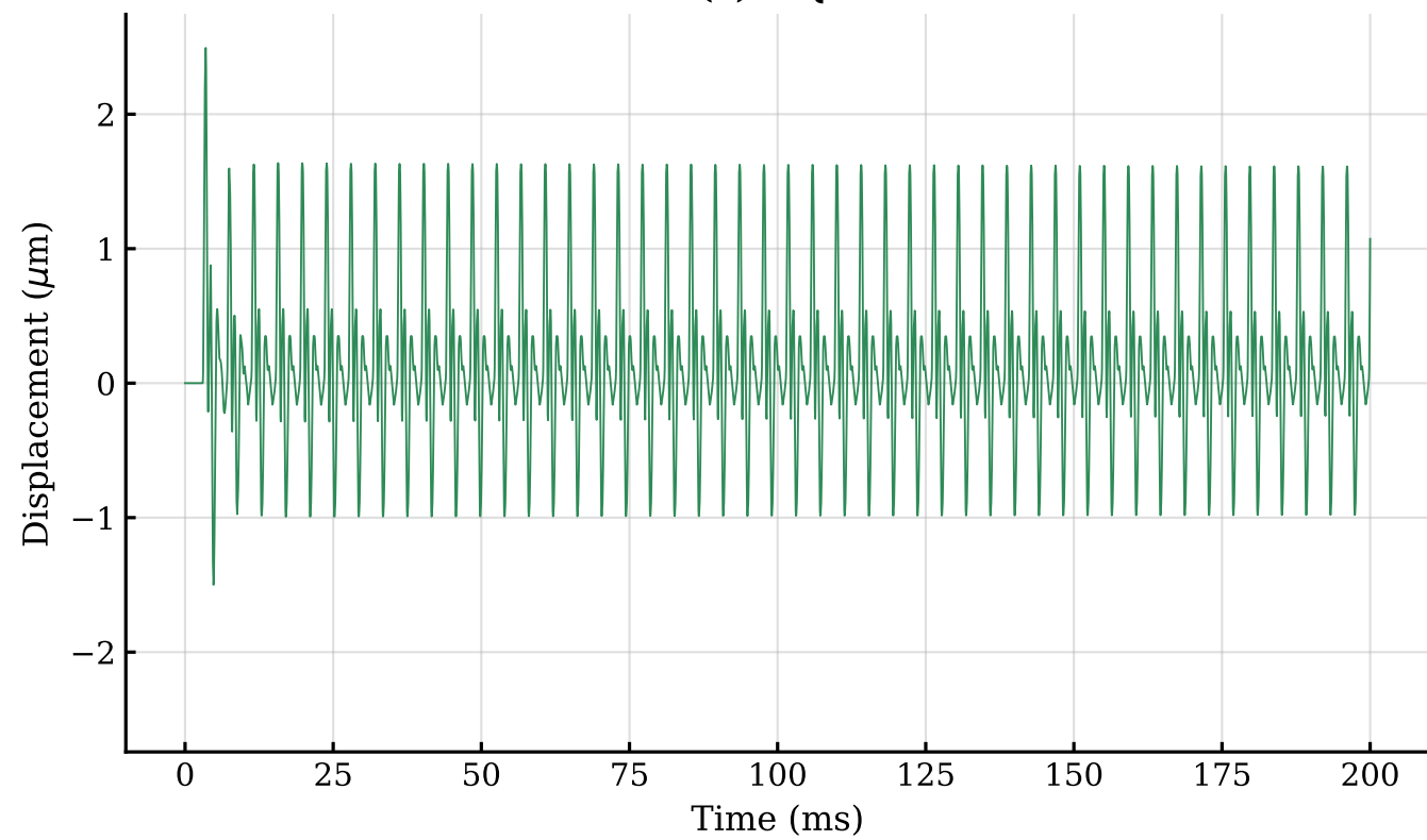
(c) FFT[LQG]
