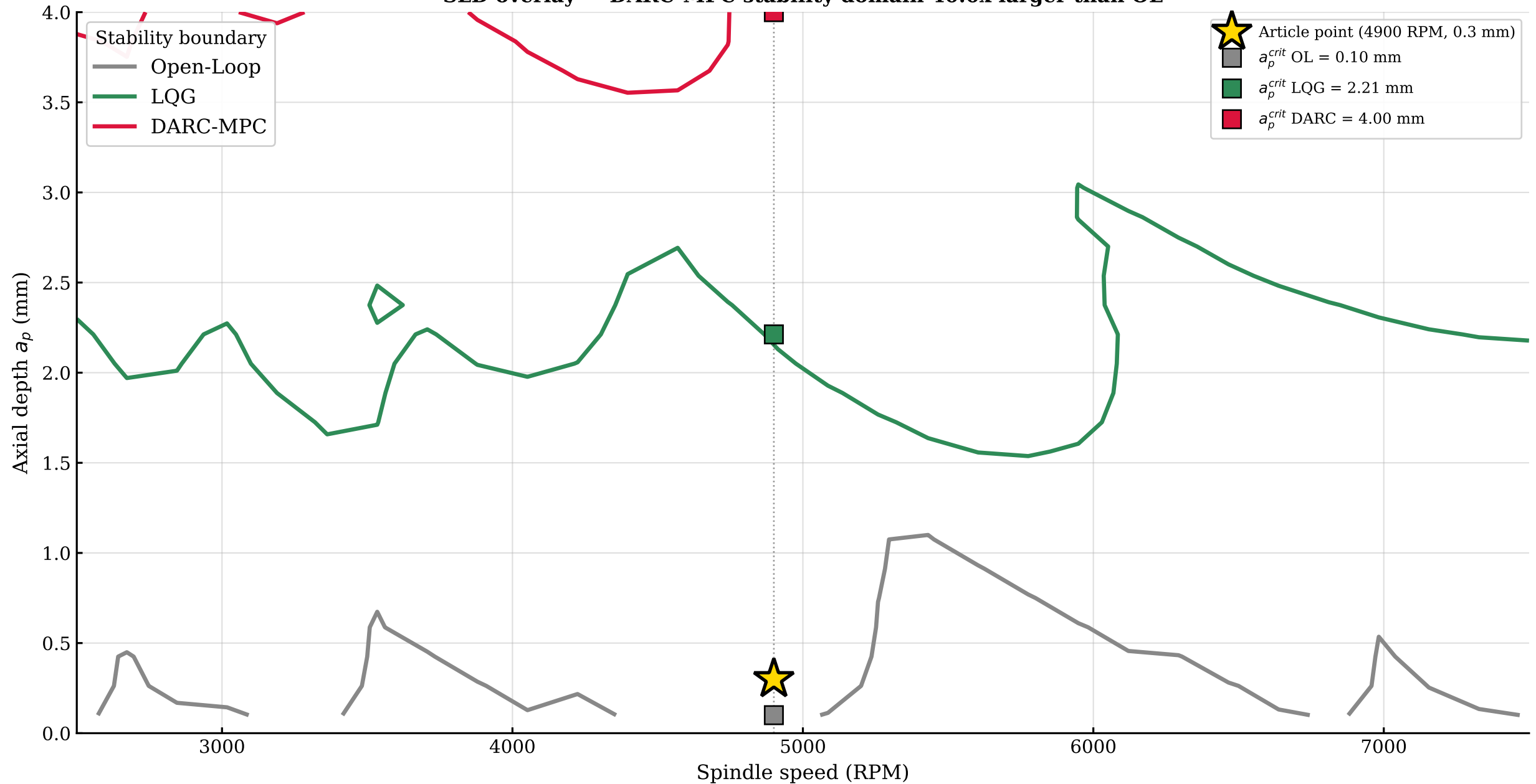
SLD overlay — DARC-MPC stability domain 40.0x larger than OL
