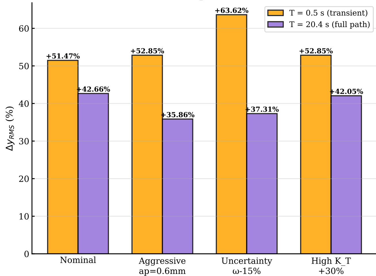
(a) DARC-MPC improvement over LQG
