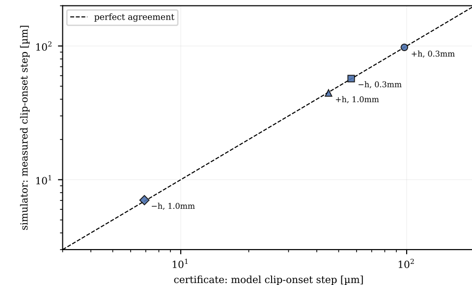
(c) certificate vs nonlinear simulator (0.02–1.9 %)
