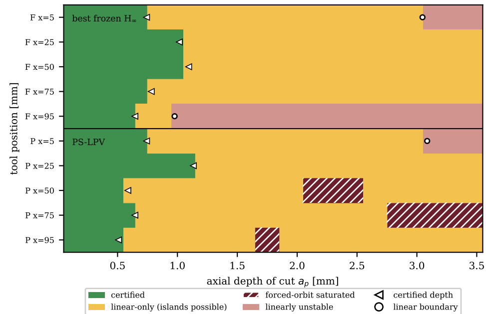
(c) certificate vs nonlinear simulator (0.02–1.9 %)
