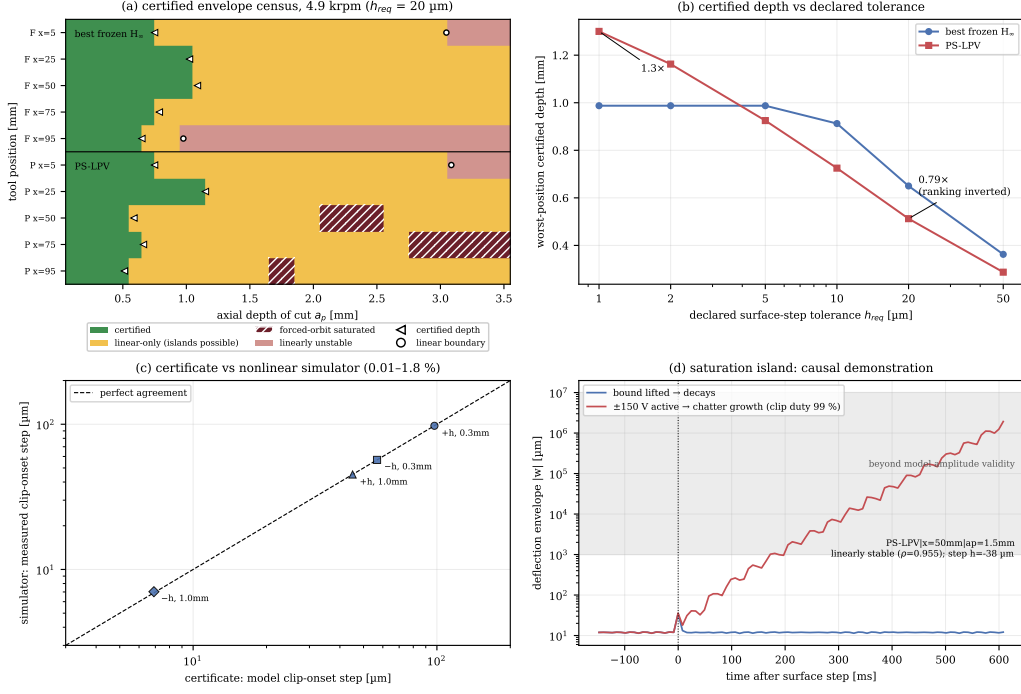
Figure 1: (a) Certified envelope census at 4.9krpm ( h_{req} = 20 \mu m ). (b) Worst-position certified depth vs. declared tolerance: the ranking inversion. (c) Certificate vs. nonlinear-simulator clip onset (parity, both signs). (d) Saturation island, causal demonstration: the same -38 \mu m step decays with the bound lifted and grows into chatter at 99% clip duty with the \pm 150 V bound active.
