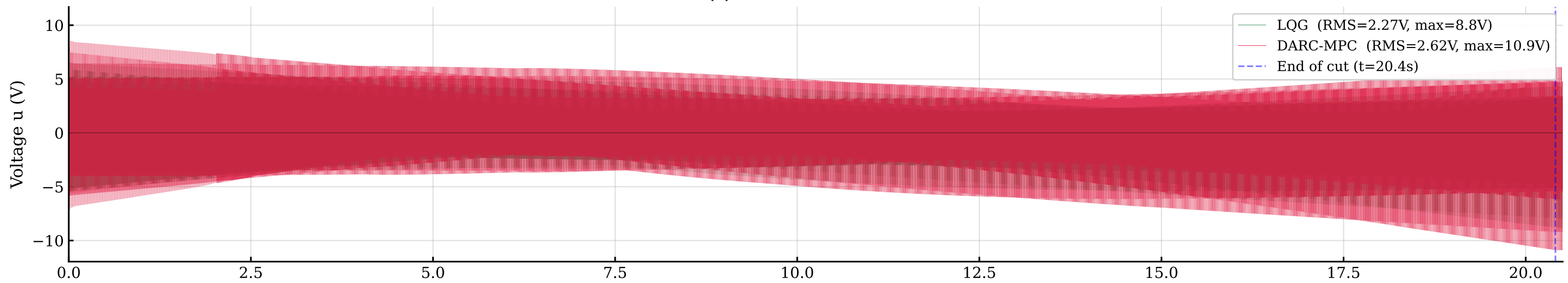
(b) S2 - Aggressive a_p=0.6 mm
