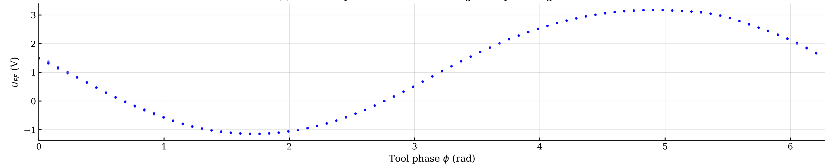
(c) Learned periodic feedforward signal — phase signature
