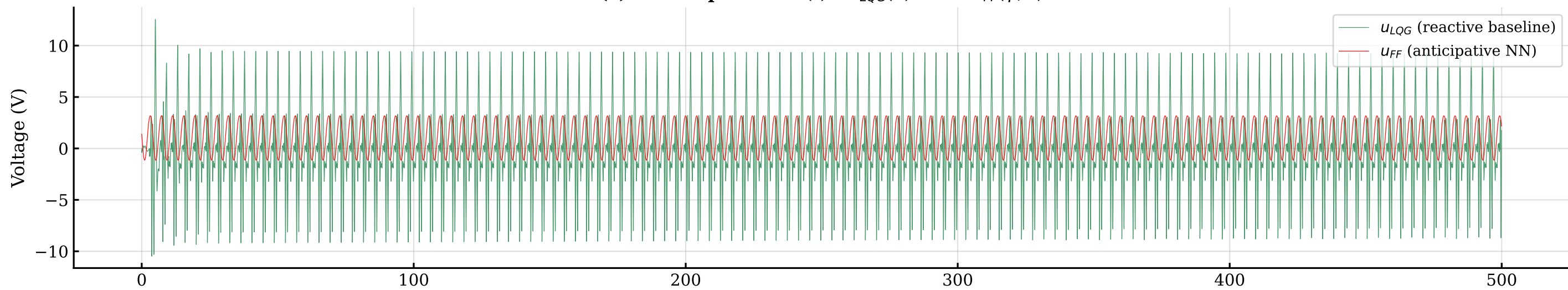
(b) Total applied voltage (max = 11.48 V)
