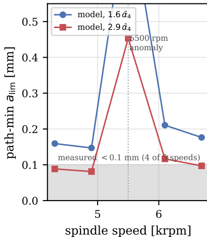
(b) open-loop limit vs measured
