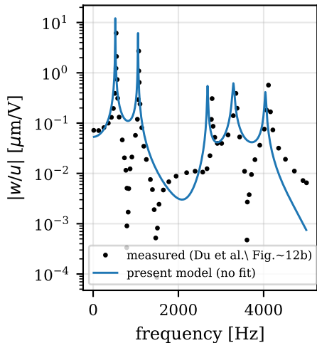
(a) actuator FRF vs measured
