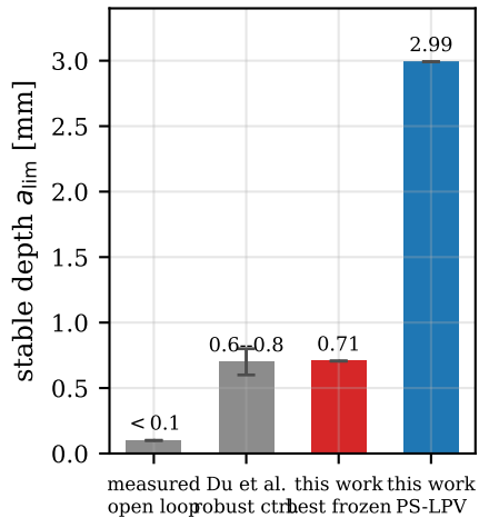
(c) stable depth benchmark
