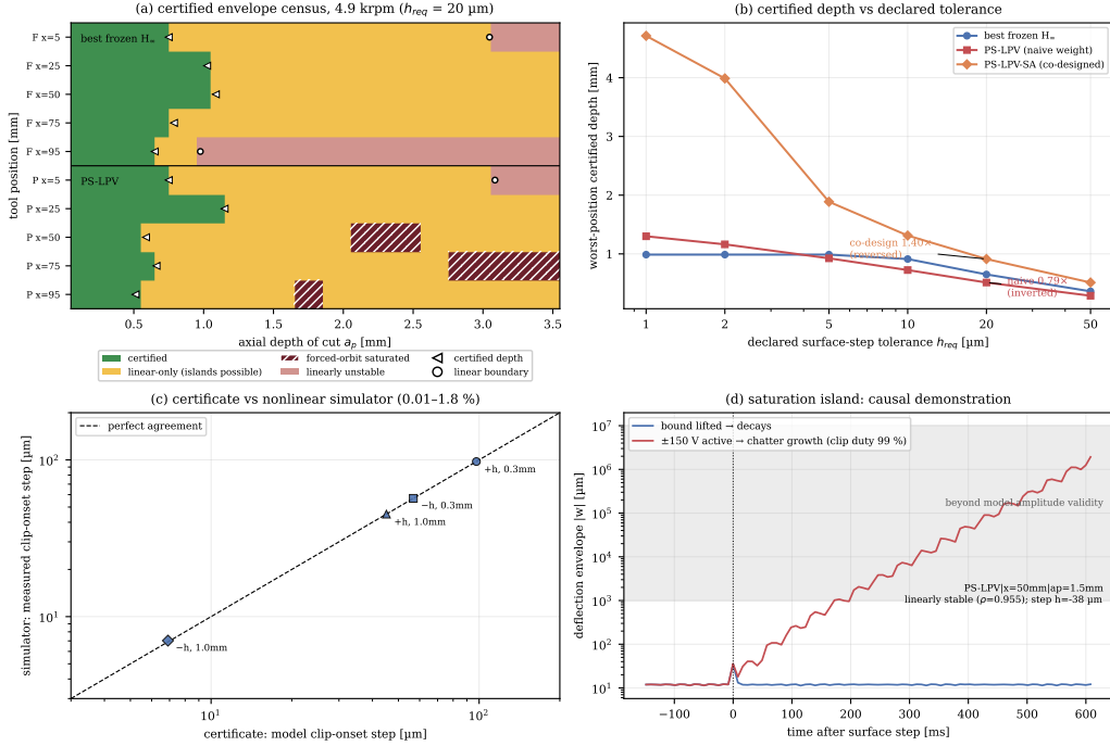
Figure 16: Saturation-aware certification at 4900 rpm. (a) Certified envelope census ( h_{\text{req}} = 20 \mu\text{m} ): certified / linear-only / forced-saturated / unstable zones for the frozen and naively weighted scheduled designs (the forced-saturated and island-prone zones appear only for the naive schedule). (b) Worst-position certified depth versus declared surface-defect tolerance: the naive schedule inverts below the frozen design, and the co-designed schedule (Section 6.6) reverses the inversion at every tolerance. (c) Certificate versus nonlinear-simulator clip onset, both step signs. (d) Saturation island, causal demonstration: the same -38 \mu\text{m} step decays with the amplifier bound lifted and grows into chatter at 99% clip duty with the \pm 150 \text{ V} bound active.
