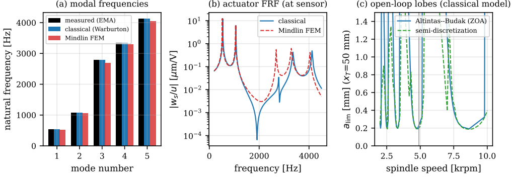
Figure 4: Independent classical-model cross-validation. (a) Modal frequencies: the classical Warburton model (anchored to the measured EMA) against the Mindlin finite-element model and the measured values. (b) Voltage-to-displacement receptance at the sensor: classical versus finite-element (overlapping at the two dominant modes). (c) Open-loop stability lobes at x_T = 50 mm: the classical Altintas–Budak zero-order solution against the semi-discretization limit on the same classical model; the lobe minima coincide, and the zero-order solution over-predicts off-lobe at this low radial immersion ( a_e/D = 0.01 ).
