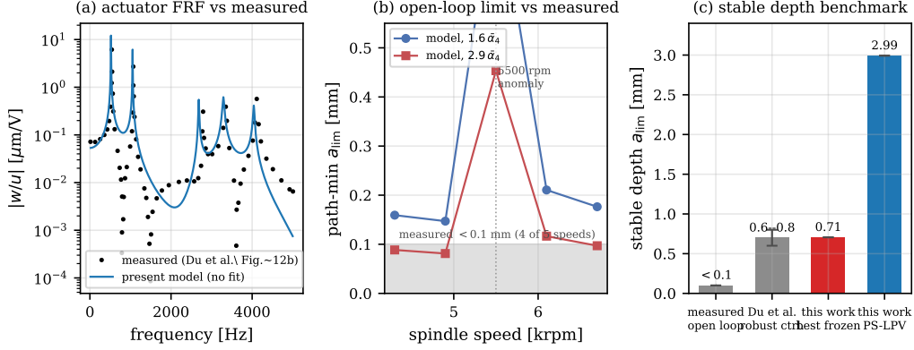
Figure 10: Direct benchmark against the reference rig [13]. (a) Actuator voltage-to-displacement FRF: present model (absolute, no fit) through the digitized measured points (their Fig. 12b). (b) Open-loop path-minimum critical depth across the five tested spindle speeds at the reference’s calibrated coefficient scalings, against their measured band. (c) Stable depth of cut: measured open loop and the reference’s non-scheduled robust controller (0.6–0.8 mm), against the present best-frozen and scheduled designs on the same hardware.
