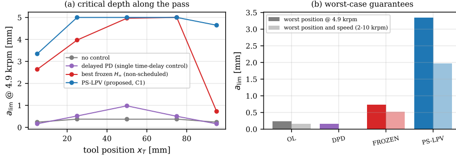
Figure 9: Critical depth of cut at 4900 rpm as a function of tool position: the frozen controller’s authority collapses toward the ends of the pass; the scheduled controller sustains it along the entire path.
