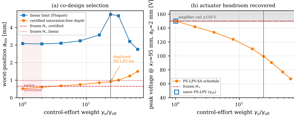
Figure 17: Saturation-aware co-design at 4900 rpm. (a) Worst-position certified saturation-free depth and linear (Floquet) limit versus the control-effort weight \gamma_u/\gamma_{u0} ( \gamma_{u0} = 1/V_{\max} ). At the naive weight (multiplier 1) the certified depth dips below the frozen design—the inversion—while the linear limit has a broad interior maximum near multiplier 24 that also delivers 1.4\times the frozen certified depth. The deployed PS-LPV-SA sits at the marked weight. (b) Worst-position peak control voltage at a fixed hard cut ( x_T = 95 mm, a_p = 2 mm): the naive schedule rides the \pm 150 V rail; the co-design leaves \sim 50 V of headroom at unchanged vibration rejection.
