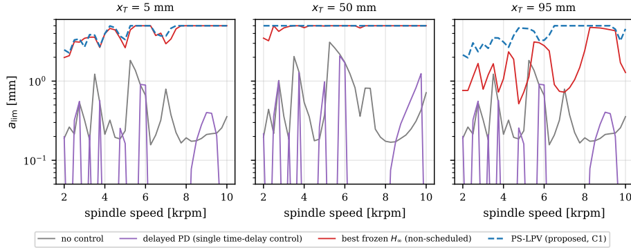
Figure 8: Closed-loop stability lobe diagrams at three tool positions on the 12-mode evaluation model: open loop, delayed PD (tuned at the reference speed; note its destabilized bands at other speeds), best-frozen H_\infty , and the scheduled PS-LPV controller. PS-LPV-DR is not drawn: its certified delayed gain is zero (Section 5.6), so it reproduces the PS-LPV lobes exactly.
