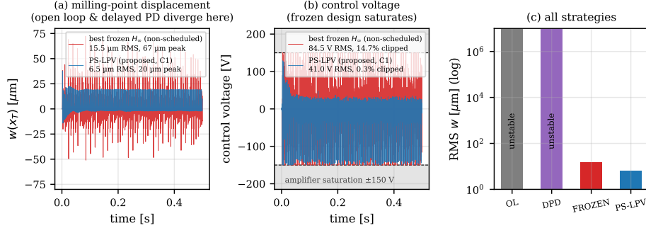
Figure 13: The differentiating condition at the end of the pass ( x_T = 95 mm, a_p = 2.0 mm, 4900 rpm): open loop and delayed PD are unstable; the frozen design survives at high amplitude and voltage; the scheduled controller is comfortable.
