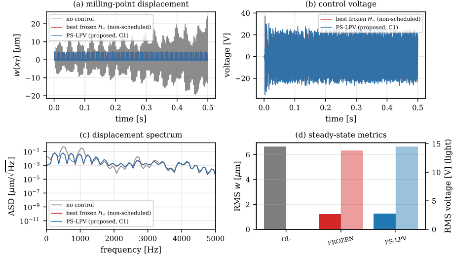
Figure 10: Time-domain response at 4900 rpm, a_p = 0.3 mm, at x_T = 5 mm—the frozen design’s own min-max design point, where the frozen and scheduled controllers coincide by construction: milling-point displacement, control voltage, spectra, and steady-state metrics. PS-LPV-DR is not drawn separately: its certified delayed gain is zero (Section 5.5), so it reproduces the PS-LPV curve exactly.
