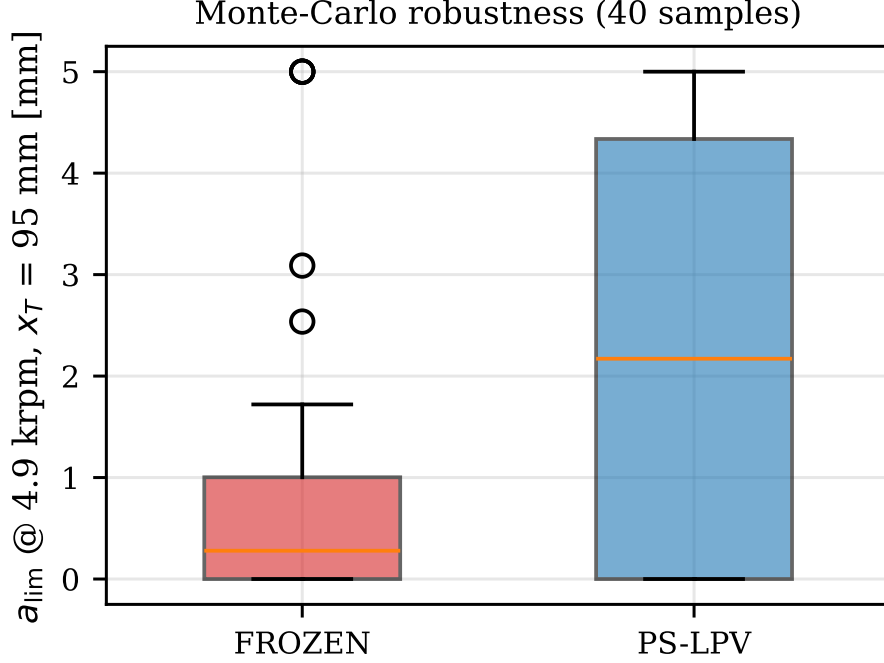
Figure 13: Robustness Monte-Carlo (40 samples, box plots) of the closed-loop critical depth at x_T = 95 mm under cutting-coefficient dispersion ( 0.3\text{--}2.9 \times \bar{\alpha}_4 ), \pm 10\% modal mass/stiffness with coherently rescaled mode shapes, and up to -20\% damping.
