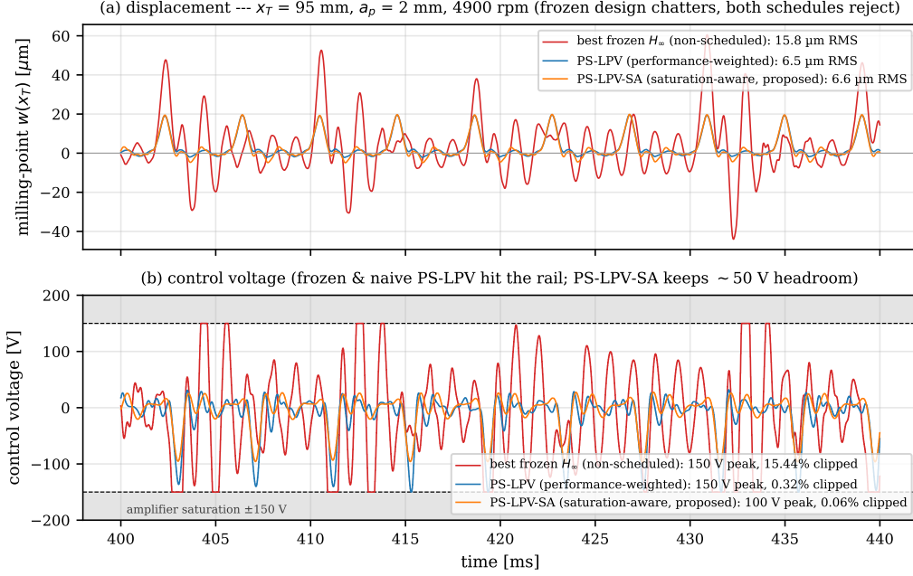
Figure 17: Time-domain response at the hard end-of-pass condition ( x_T = 95 mm, a_p = 2 mm, 4900 rpm), steady-state window. (a) Milling-point displacement: the frozen H_\infty design chatters at 15.8 \mu\text{m} RMS, while both the naive and the saturation-aware schedules reject it to \sim 6.5 \mu\text{m} RMS (their traces nearly coincide). (b) Control voltage: the frozen design and the naive PS-LPV both reach the \pm 150 V rail (15.4% and 0.32% of the time), whereas the co-designed PS-LPV-SA achieves the same rejection with a \sim 100 V peak and 0.06% clipping—the recovered headroom of Fig. 16, made visible in the time domain.
