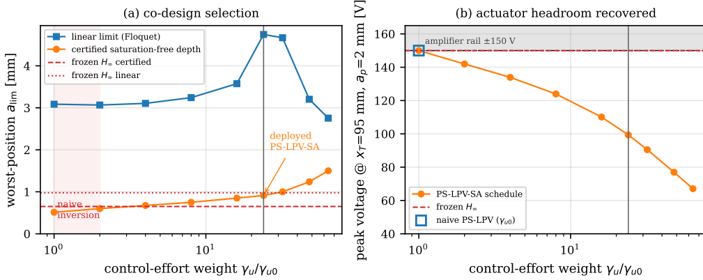
Figure 16: Saturation-aware co-design at 4900 rpm. (a) Worst-position certified saturation-free depth and linear (Floquet) limit versus the control-effort weight \gamma_u/\gamma_{u0} ( \gamma_{u0} = 1/V_{\max} ). At the naive weight (multiplier 1) the certified depth dips below the frozen design—the inversion—while the linear limit has a broad interior maximum near multiplier 24 that also delivers 1.4\times the frozen certified depth. The deployed PS-LPV-SA sits at the marked weight. (b) Worst-position peak control voltage at a fixed hard cut ( x_T = 95 mm, a_p = 2 mm): the naive schedule rides the \pm 150 V rail; the co-design leaves \sim 50 V of headroom at unchanged vibration rejection.
