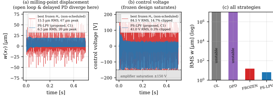
Figure 12: The differentiating condition at the end of the pass ( x_T = 95 mm, a_p = 2.0 mm, 4900 rpm): open loop and delayed PD are unstable; the frozen design survives at high amplitude and voltage; the scheduled controller is comfortable.
