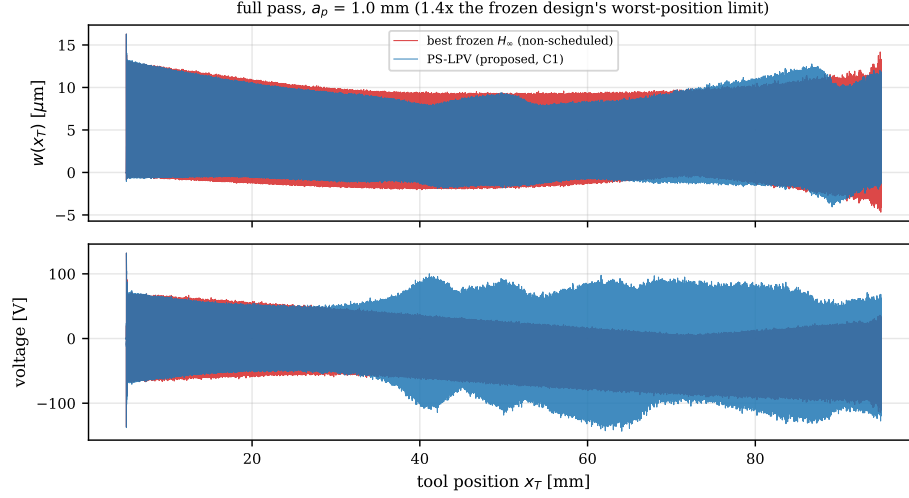
Figure 11: Full moving pass (20.4 s) at a_p = 1.0 mm with continuously updated scheduled gains: milling-point displacement and control voltage against tool position, best-frozen H_\infty versus scheduled PS-LPV.
