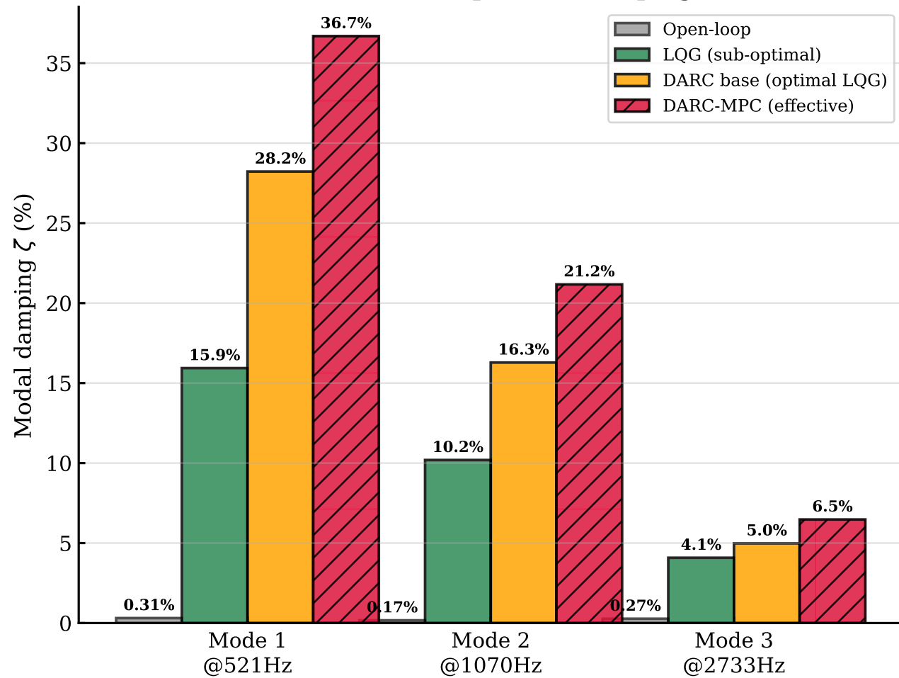
(a) Closed-loop modal damping
