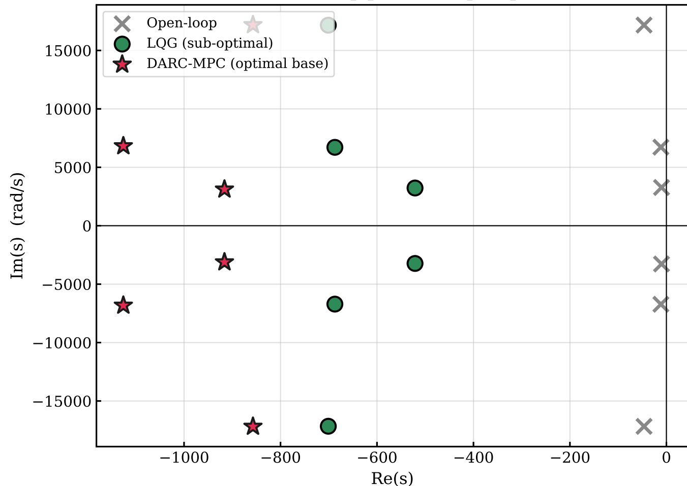
(b) Closed-loop poles (complex plane)
