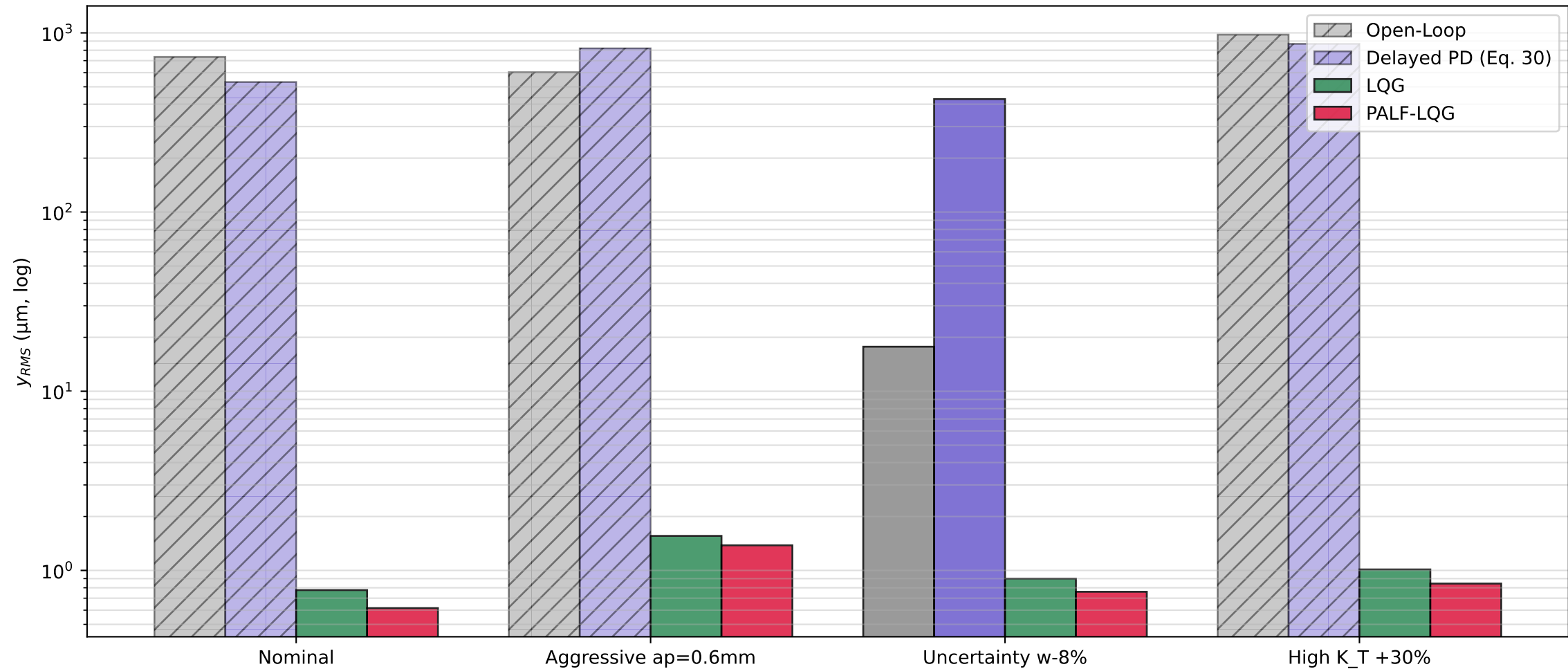
Four-way benchmark (hatched = diverged): OL / Delayed PD / LQG / PALF-LQG
