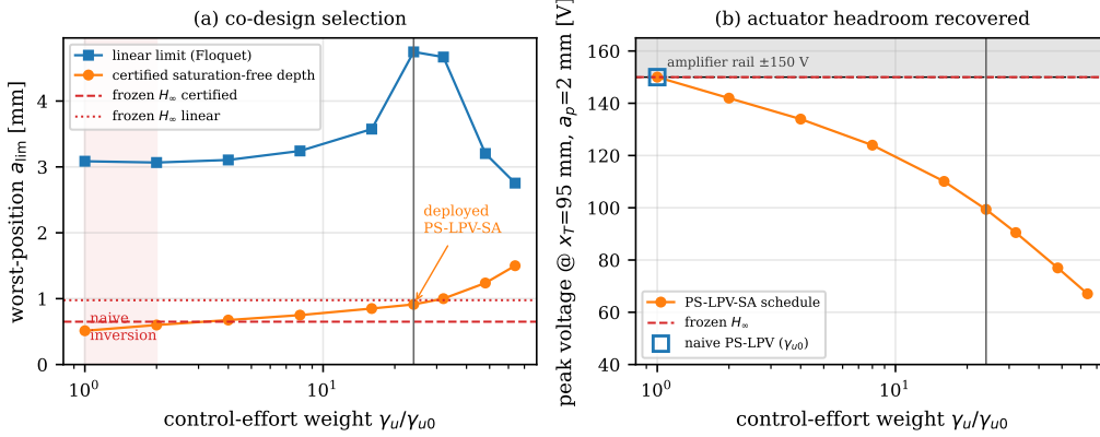
Figure 15: Saturation-aware co-design at 4900 rpm. (a) Worst-position certified saturation-free depth and linear (Floquet) limit versus the control-effort weight \gamma_u/\gamma_{u0} ( \gamma_{u0} = 1/V_{\max} ). At the naive weight (multiplier 1) the certified depth dips below the frozen design—the inversion—while the linear limit has a broad interior maximum near multiplier 24 that also delivers 1.4\times the frozen certified depth. The deployed PS-LPV-SA sits at the marked weight. (b) Worst-position peak control voltage at a fixed hard cut ( x_T = 95 mm, a_p = 2 mm): the naive schedule rides the \pm 150 V rail; the co-design leaves \sim 50 V of headroom at unchanged vibration rejection.
