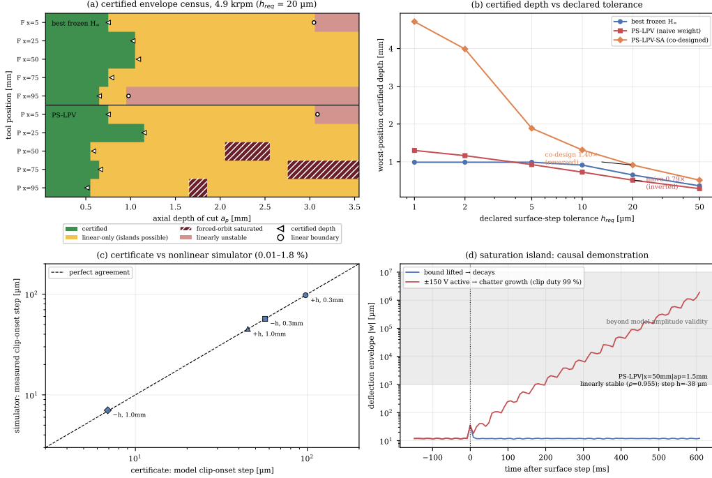
Figure 14: Saturation-aware certification at 4900 rpm. (a) Certified envelope census ( h_{\text{req}} = 20 \mu\text{m} ): certified / linear-only / forced-saturated / unstable zones for the frozen and naively weighted scheduled designs (the forced-saturated and island-prone zones appear only for the naive schedule). (b) Worst-position certified depth versus declared surface-defect tolerance: the naive schedule inverts below the frozen design, and the co-designed schedule (Section 6.6) reverses the inversion at every tolerance. (c) Certificate versus nonlinear-simulator clip onset, both step signs. (d) Saturation island, causal demonstration: the same -38 \mu\text{m} step decays with the amplifier bound lifted and grows into chatter at 99% clip duty with the \pm 150 \text{ V} bound active.
