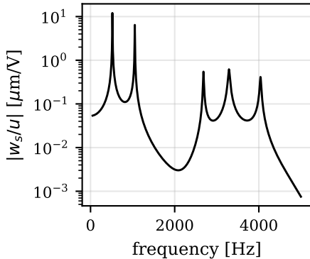
(b) actuator authority
