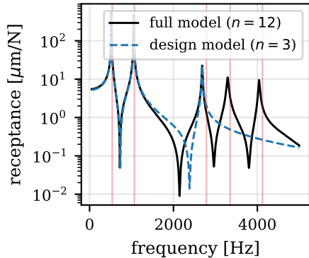
(a) tip receptance
