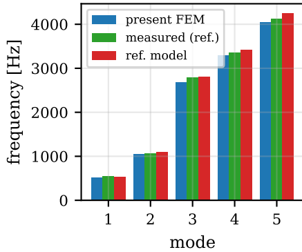
(c) natural frequencies
