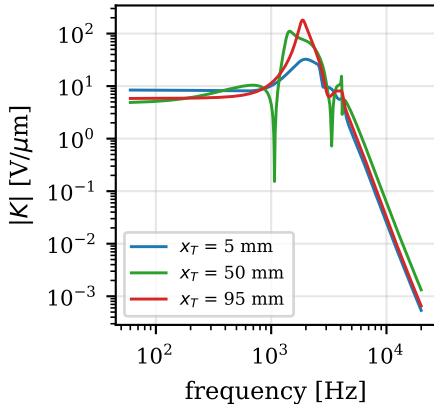
(b) deployed scheduled controller
