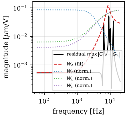
(a) uncertainty overbound and weights
