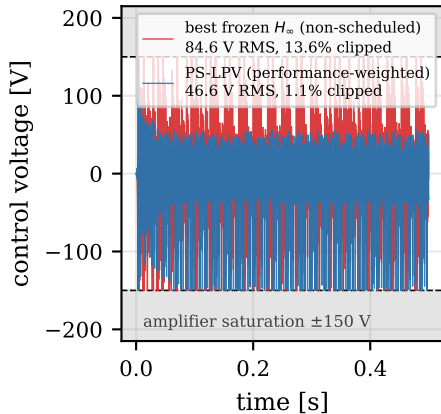
(b) control voltage (frozen design saturates)
