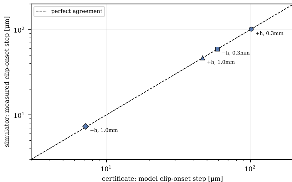
(c) certificate vs nonlinear simulator (0.01–2.0 %)
