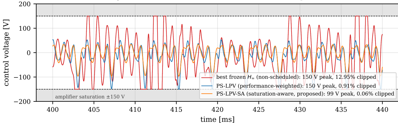
(b) control voltage (frozen & naive PS-LPV hit the rail; PS-LPV-SA keeps \sim 50 V headroom)
