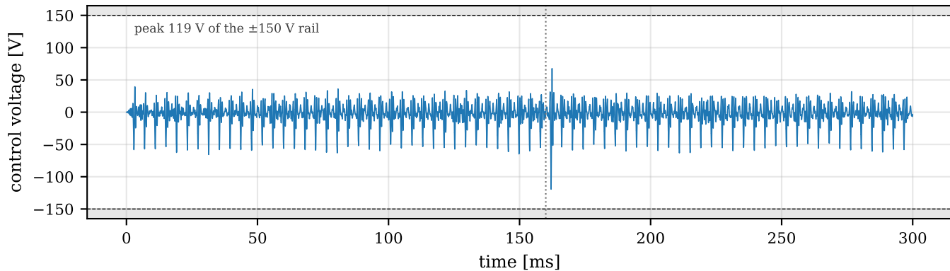
(b) control voltage (the controller's response)
