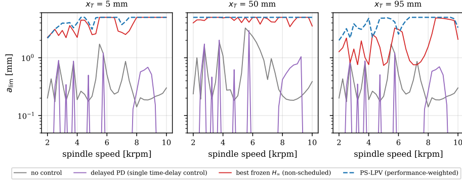
Figure 8: Closed-loop stability lobe diagrams at three tool positions on the 12-mode evaluation model: open loop, delayed PD (tuned at the reference speed; note its destabilized bands at other speeds), best-frozen H_\infty , and the scheduled PS-LPV controller. PS-LPV-DR is not drawn: its certified delayed gain is zero (Section 5.6), so it reproduces the PS-LPV lobes exactly.
