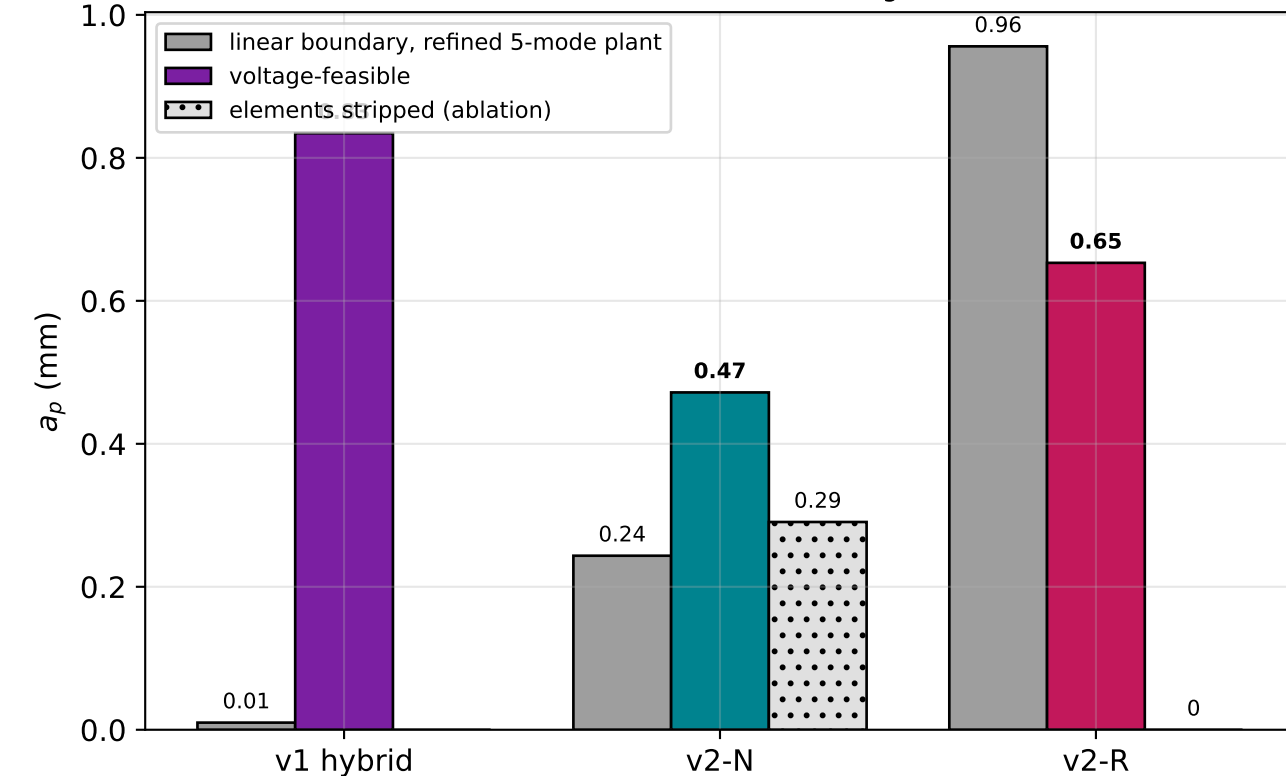
(d) spillover repair (refined-plant linear boundary 0.01 \rightarrow 0.96 mm) and load-bearing ablation
