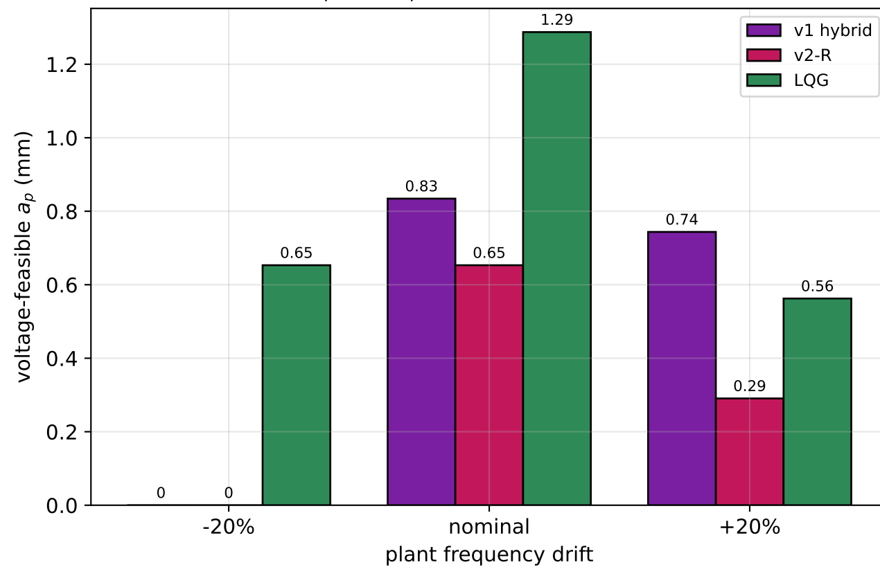
(c) drift robustness: the -20% weakness persists on the refined plant despite the linear min-max certificate
