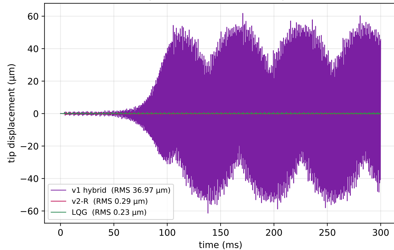
(d) spillover repair (refined-plant linear boundary 0.01 \rightarrow 0.96 mm) and load-bearing ablation
