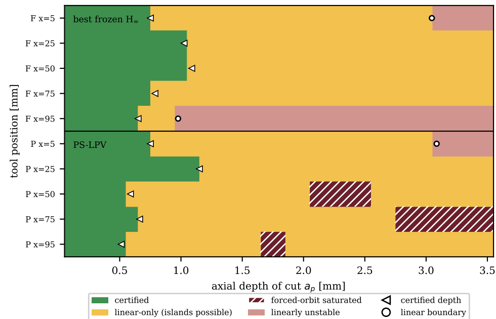
(c) certificate vs nonlinear simulator (0.01–1.8 %)
