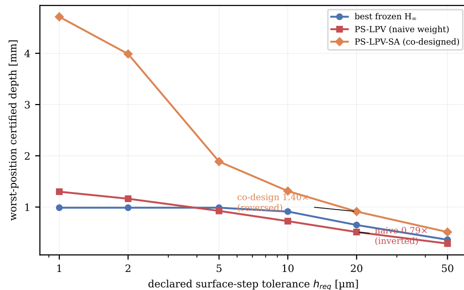
(b) certified depth vs declared tolerance
