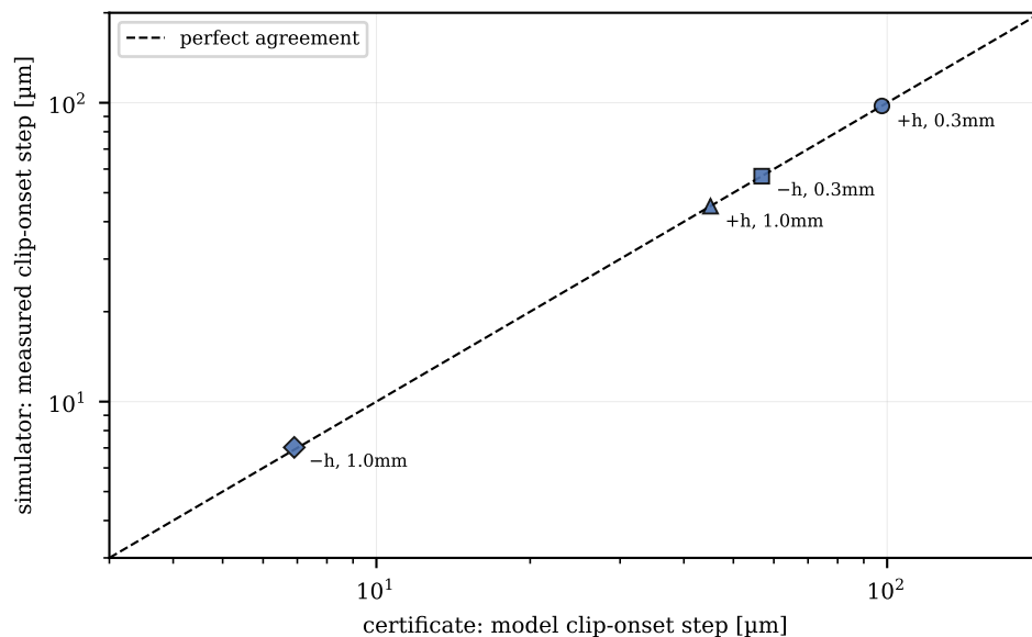
(c) certificate vs nonlinear simulator (0.01–1.8 %)
