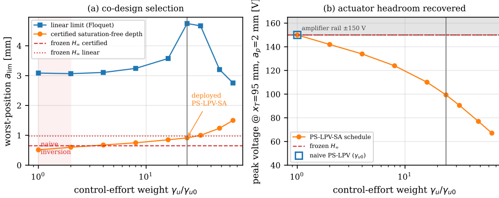
Figure 15: Saturation-aware co-design at 4900 rpm. (a) Worst-position certified saturation-free depth and linear (Floquet) limit versus the control-effort weight \gamma_u/\gamma_{u0} ( \gamma_{u0} = 1/V_{\max} ). At the naive weight (multiplier 1) the certified depth dips below the frozen design—the inversion—while the linear limit has a broad interior maximum near multiplier 24 that also delivers 1.4\times the frozen certified depth. The deployed PS-LPV-SA sits at the marked weight. (b) Worst-position peak control voltage at a fixed hard cut ( x_T = 95 mm, a_p = 2 mm): the naive schedule rides the \pm 150 V rail; the co-design leaves \sim 50 V of headroom at unchanged vibration rejection.
