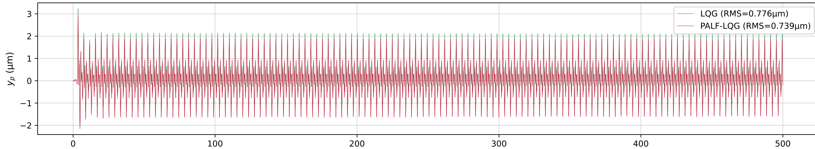
S2 - Aggressive ap=0.6mm
