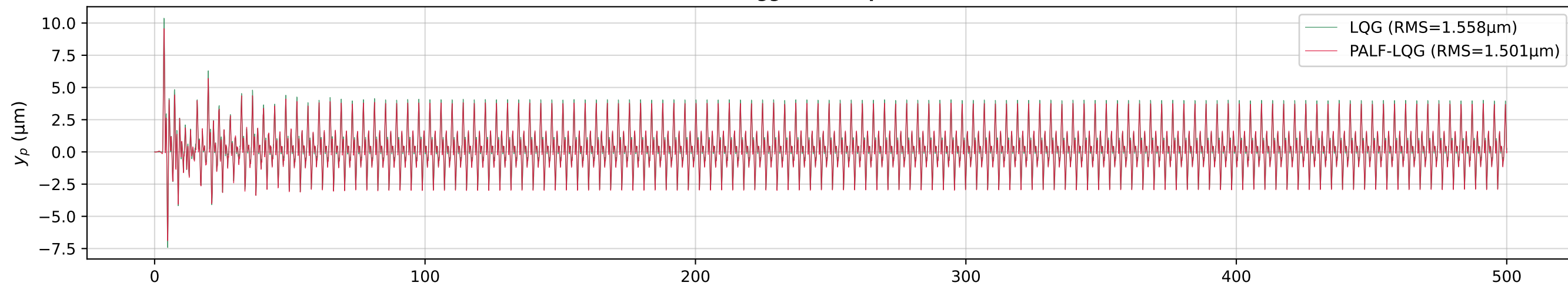
S3 - Uncertainty \omega -8%
