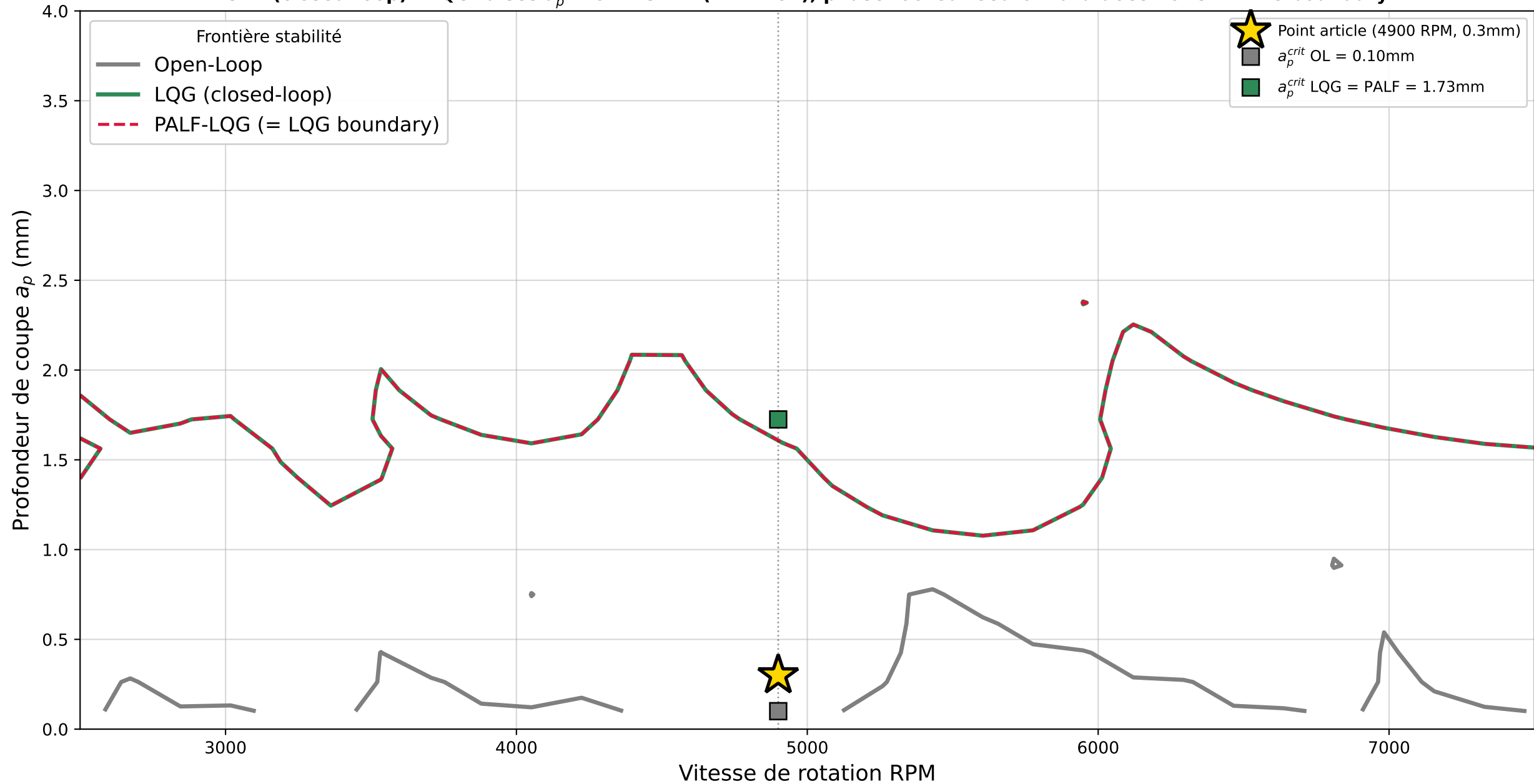
SLD (closed-loop) - LQG raises a_p^{crit} to 1.73mm (17.2x OL); phase-locked feedforward does not shift the boundary
