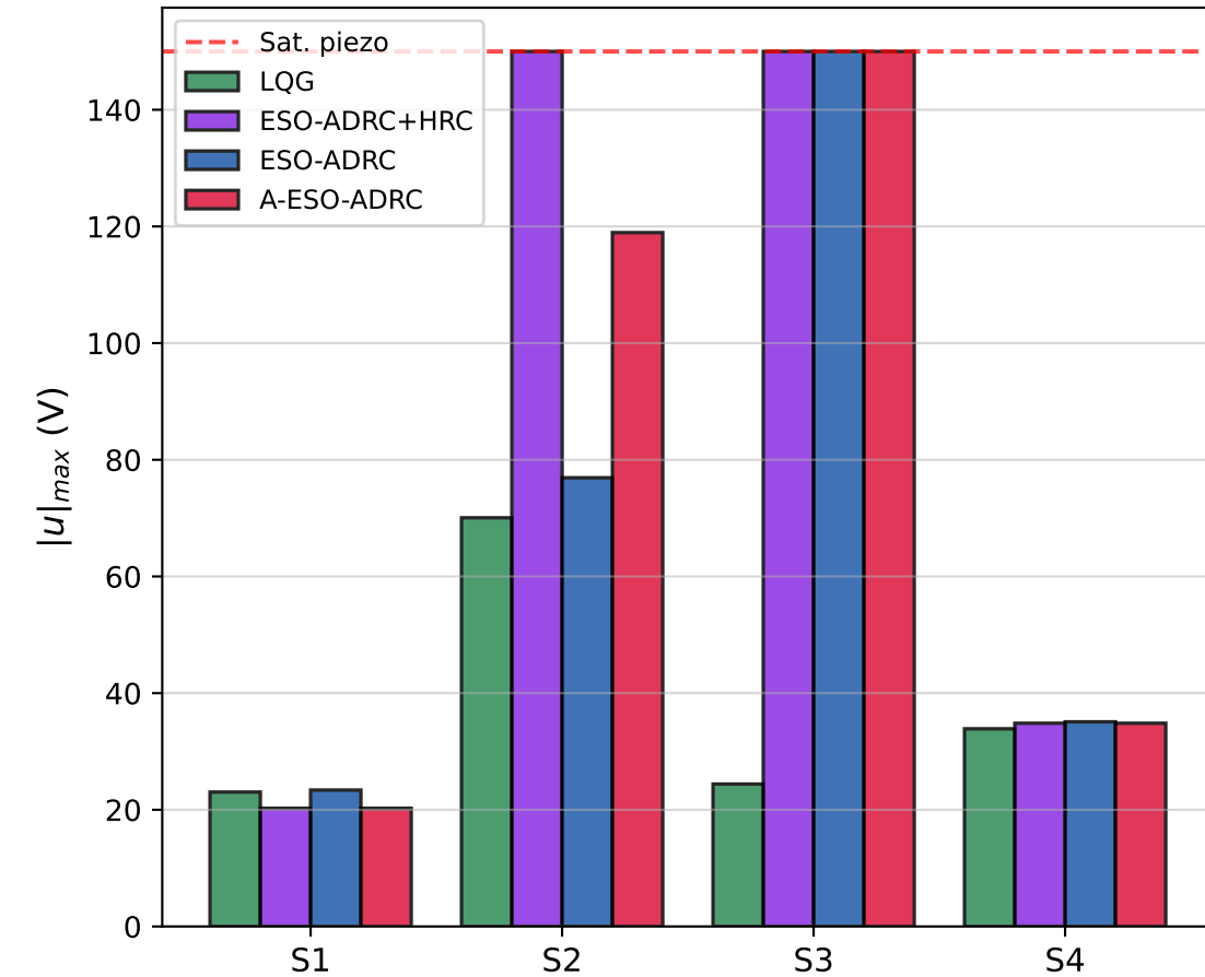
Peak control effort
