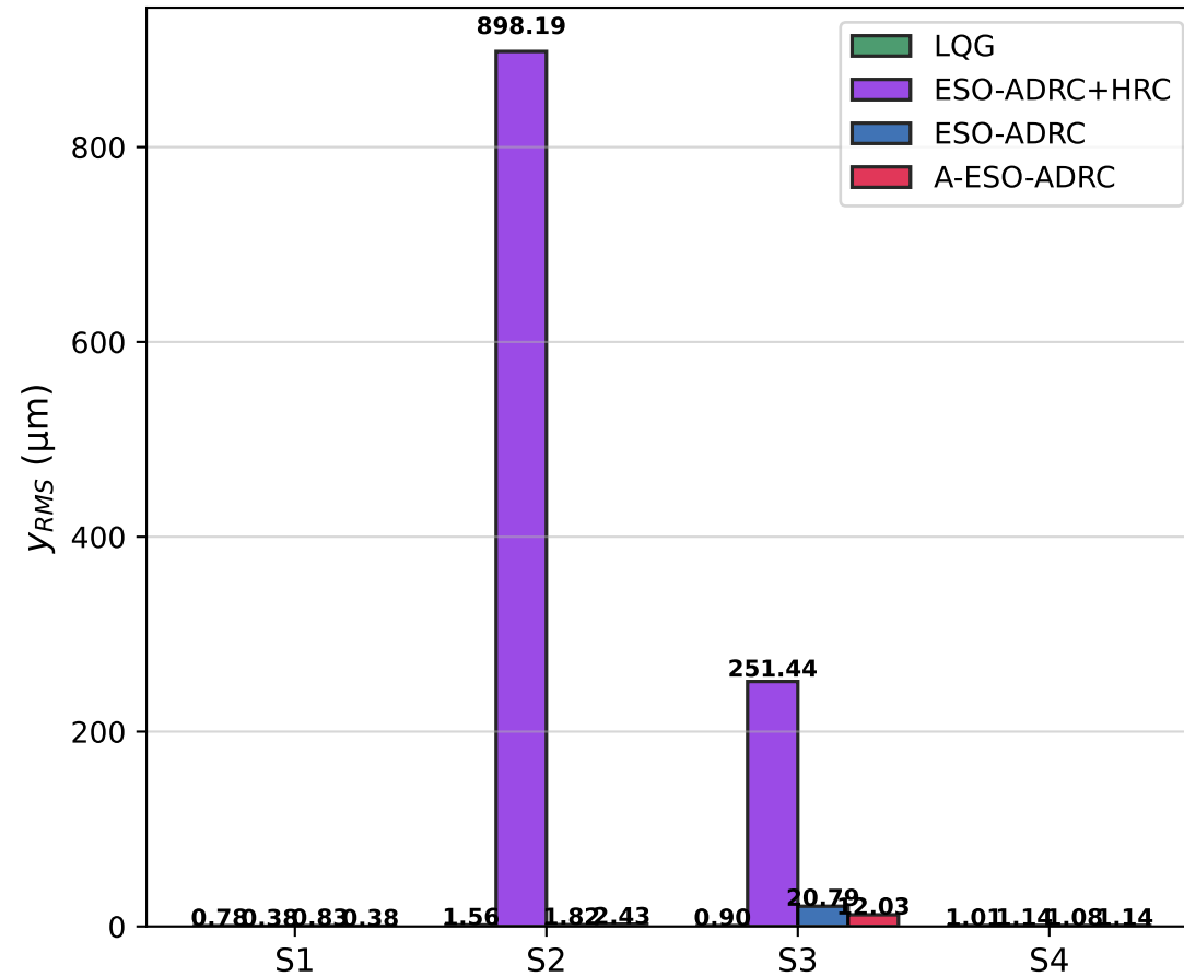
Vibration RMS
