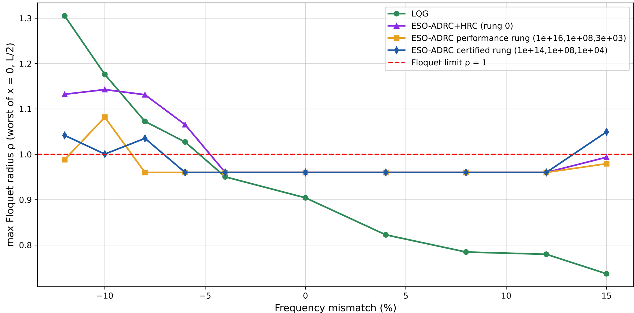
Design-time certification: closed-loop monodromy over the mismatch ball ( a_p = 0.3 mm, 4900 RPM — complementary robustness of the two rungs motivates the supervised ladder)
