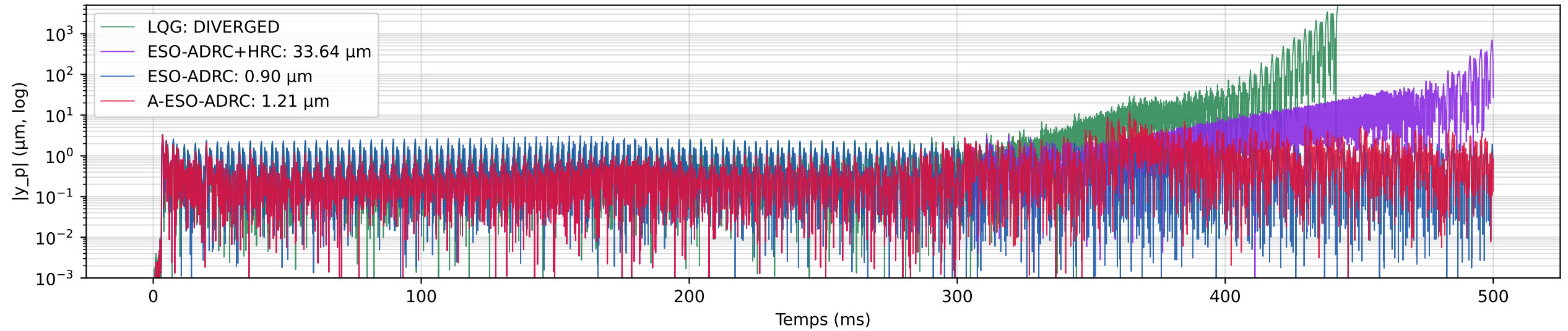
D2 ramp -12% — frequency drift DURING the pass (ramp over 60 %, then hold)
