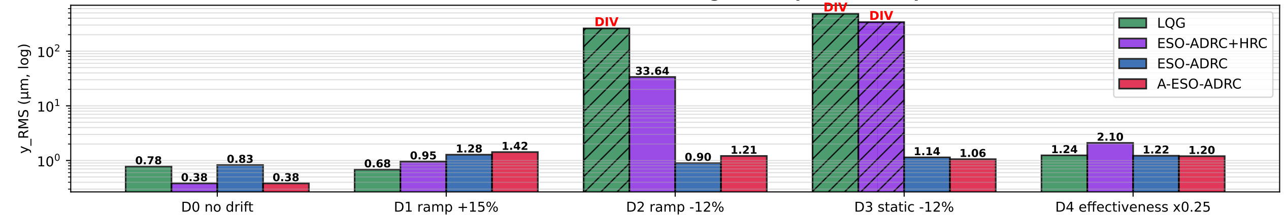
Drift / stress benchmark — fixed designs vs supervised adaptation
