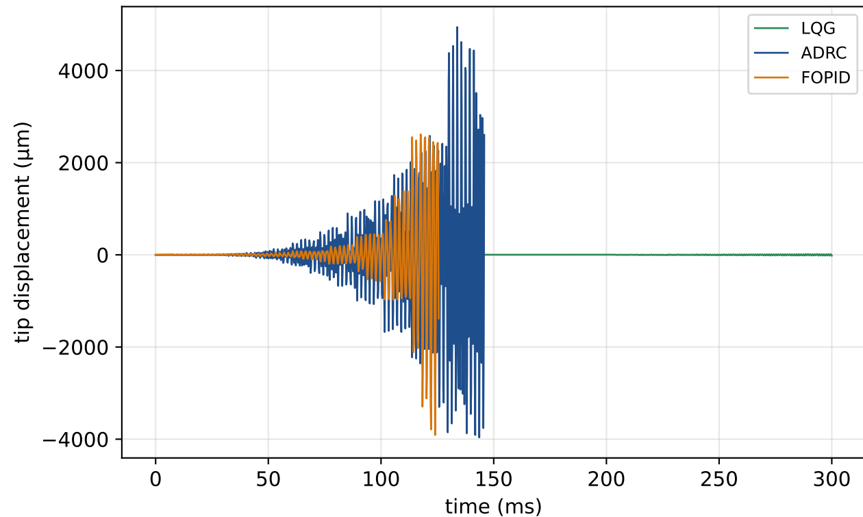
(b) tip response at a_p = 0.5 mm on the tip sensor diverging traces terminate at the chatter threshold
