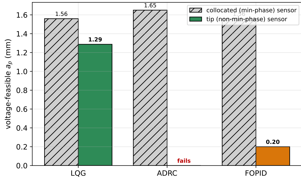
(a) feasible depth on the common tip sensor ADRC fails on the NMP tip; FOPID degrades; LQG least affected
