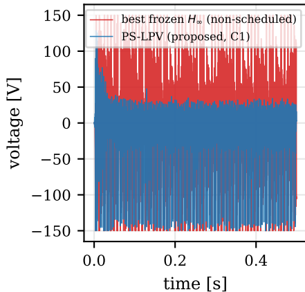
(b) control voltage
