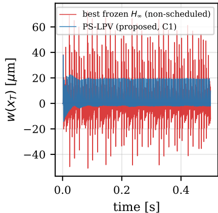
(a) displacement (stable pair)
