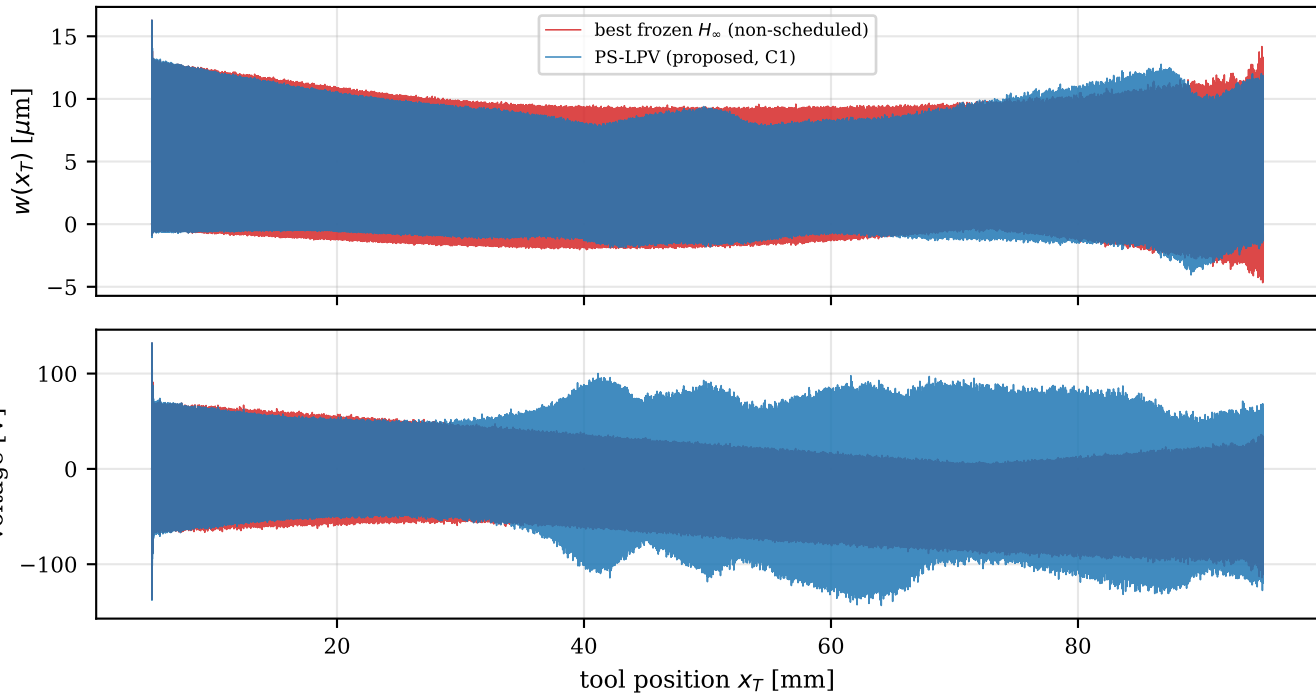
full pass, a_p = 1.0 mm (1.4x the frozen design's worst-position limit)
