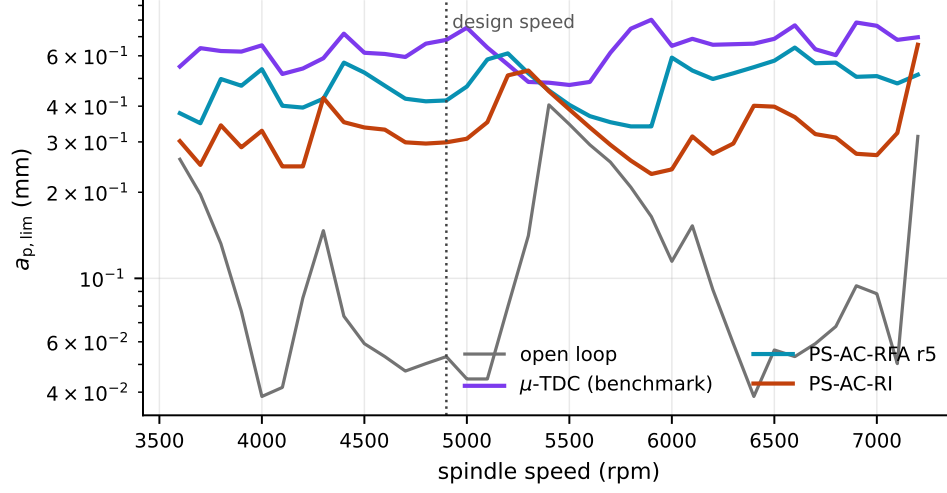
Figure 5: Stability lobes: critical depth of cut vs. spindle speed, minimum over the tool-path positions \{0, L/2, L\} (five-mode truth model, Floquet m = 120 , bisection to 5 \mu\text{m} ). The dotted line marks the design speed. Source: lobes.npz .
