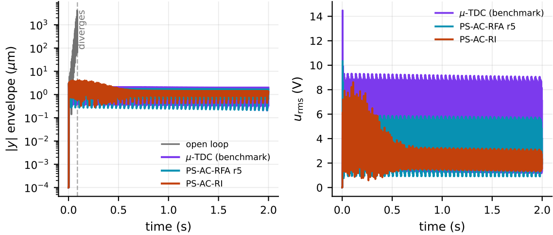
Figure 6: Time response at the reference condition (4900 rpm, a_p = 0.3 \text{ mm} , moving cut, 2 s window). Left: displacement envelope at the sensor (log scale)—the open loop diverges at t = 0.089 \text{ s} (dashed marker); all three members hold a 3\text{--}4 \mu\text{m} peak and settle near 1 \mu\text{m} . Right: rms actuation voltage of the three members. Source: timeresp.npz .
