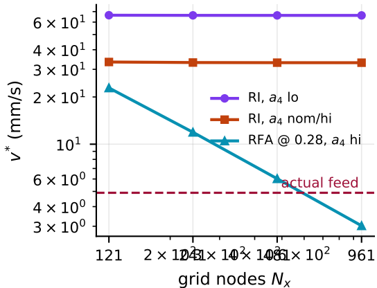
secant v^* under refinement
