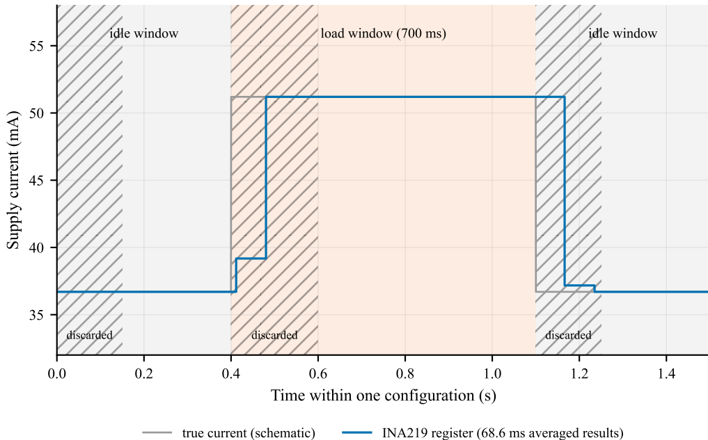
Sustained-load measurement of one configuration (schematic)
