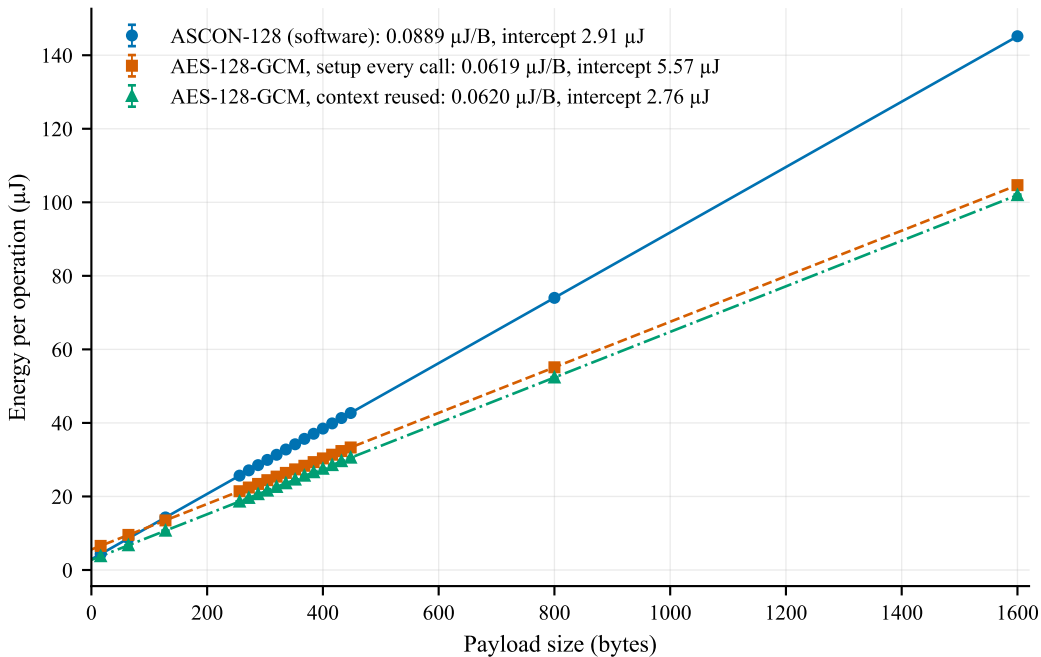
Energy per operation with linear fits (Run 1)
