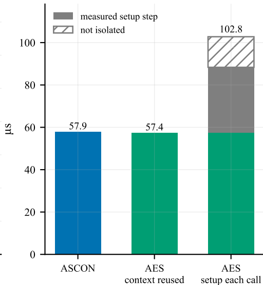
Time per operation, 16 B
