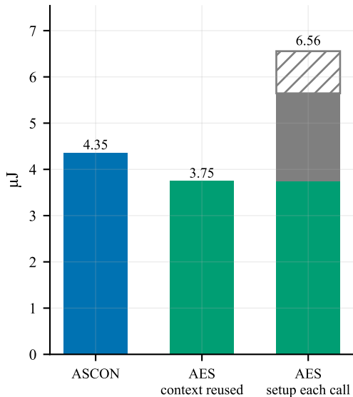
Energy per operation, 16 B
