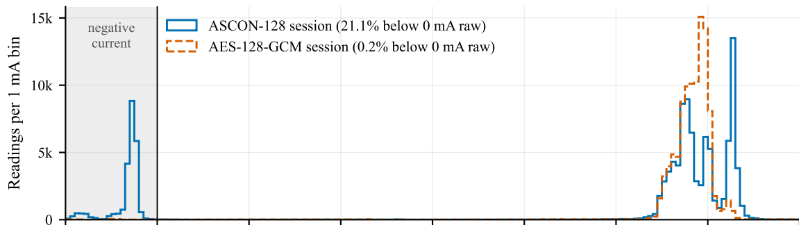
(a) Raw readings: a separate cluster below zero (median -5.6 mA)
