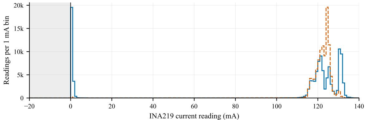
(b) After adding the 5.70 mA offset (negatives clipped to 0)
