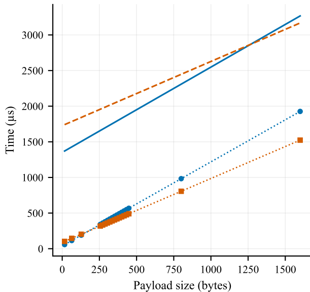
Time: constant offset in Campaign A
