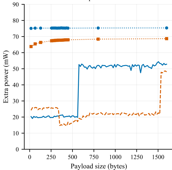
Power: steps and level differ
