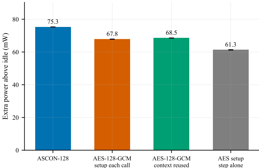
Extra power drawn while the cipher runs (payloads \geq 256 B; setup step: no payload)
