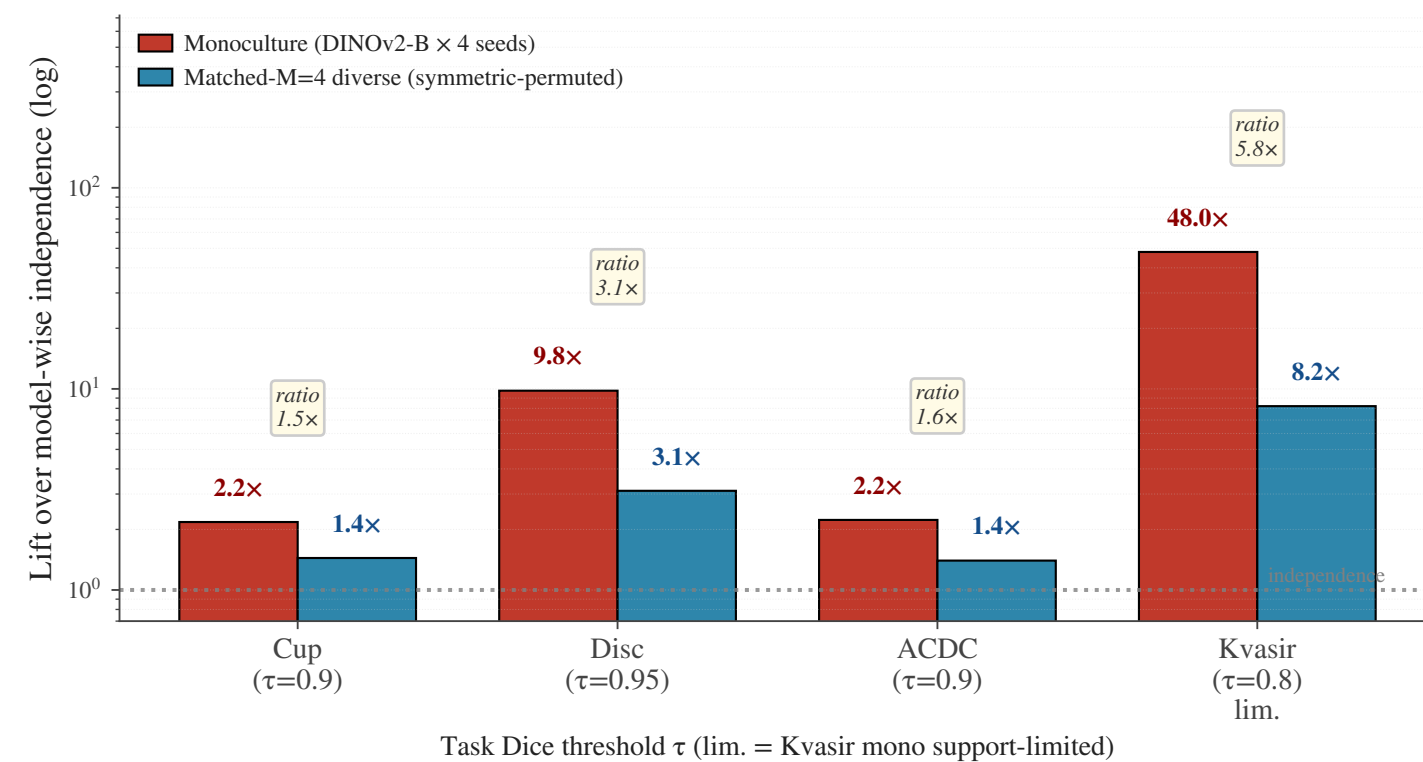
(c) Mono vs matched-M=4 lift ratios
