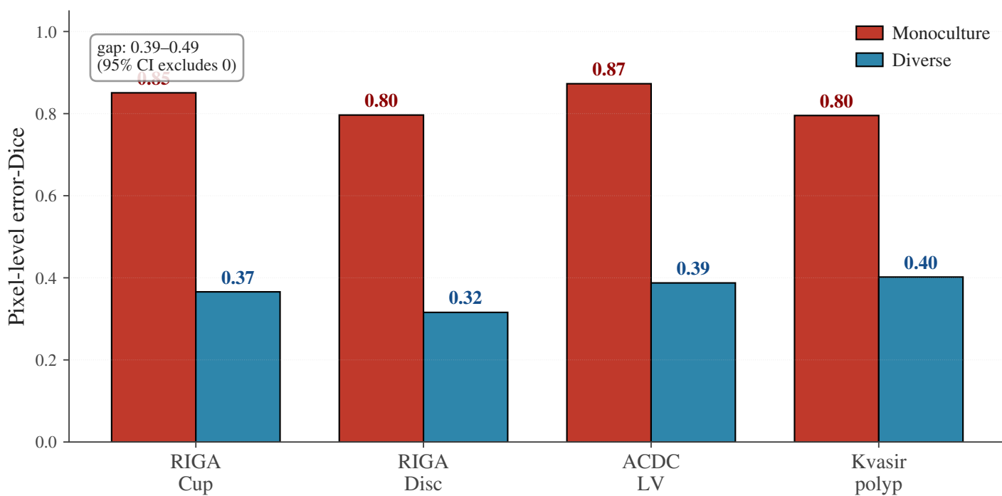
(b) Error-mask overlap across 3 domains
