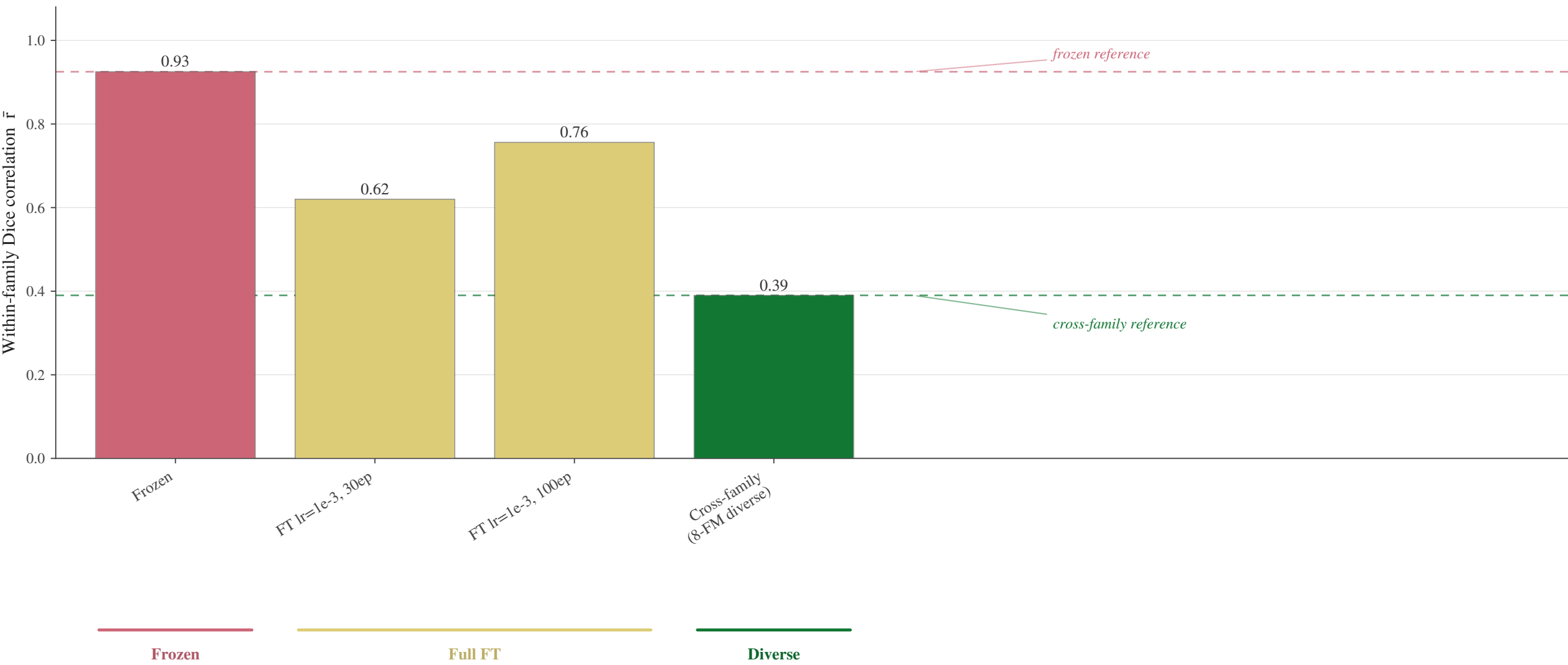
Within-family \bar{r} across adaptation regimes (RIGA Cup · DINOv2-B · 4 seeds)
