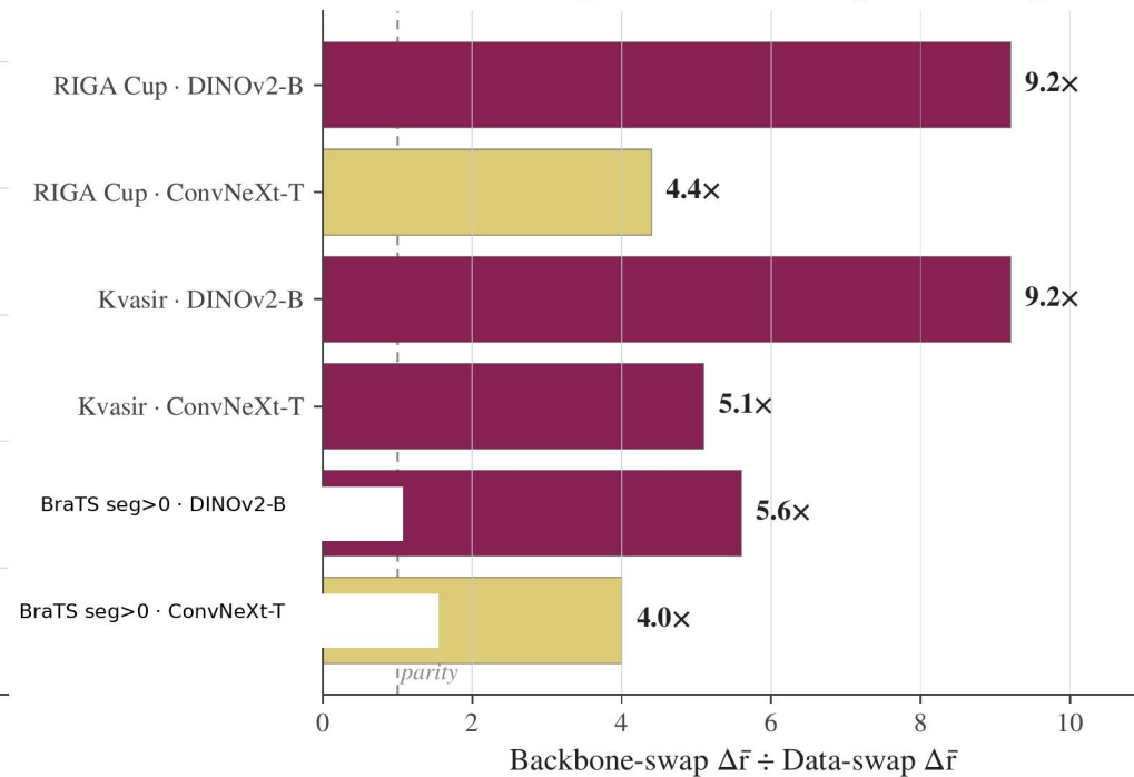
(b) Backbone swap exceeds data swap in this diagnostic
