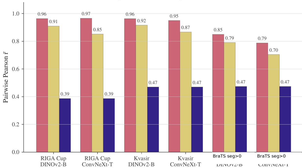
(a) Same backbone / data swap vs. backbone swap
